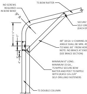
1A BOW EAVE RAFTER COLUMN CONNECTION DETAIL FOR HEIGHTS 14'-0" < TO ≤ 16'-0" SCALE: NTS
