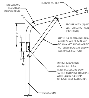
1.1 BOW EAVE RAFTER COLUMN CONNECTION DETAIL FOR HEIGHTS 12'-0" < TO ≤ 13'-0" SCALE: NTS
