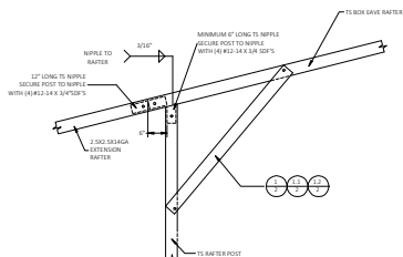
12'-0", IF THE KNEE BRACE ON THE OTHER END OF THE RAFTER IS PER DETAIL 1.2/2. 14'-0", IF THE KNEE BRACE ON THE OTHER END OF THE RAFTER IS PER DETAIL 1.1/2. 15'-0", IF THE KNEE BRACE ON THE OTHER END OF THE RAFTER IS PER DETAIL 1/2.
