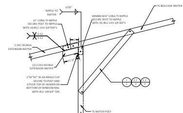
SIDE EXTENSION RAFTER/COLUMN DETAIL FOR EXTENSION RAFTER SPANS 12'-0" \leq W \leq 16'-0", IF THE KNEE BRACE ON THE OTHER END OF THE RAFTER IS PER DETAIL 1.2/2. FOR EXTENSION RAFTER SPANS 13'-0" \leq W \leq 18'-0", IF THE KNEE BRACE ON THE OTHER END OF THE RAFTER IS PER DETAIL 1.1/2. FOR EXTENSION RAFTER SPANS 15'-0" \leq W \leq 19'-0", IF THE KNEE BRACE ON THE OTHER END OF THE RAFTER IS PER DETAIL 1/2. SCALE: NTS
