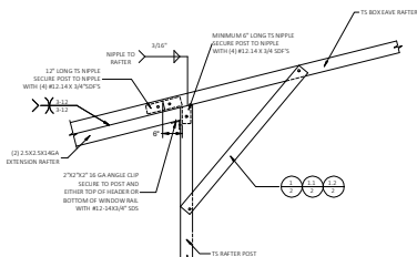
SIDE EXTENSION RAFTER/COLUMN DETAIL FOR EXTENSION RAFTER SPANS 16'-0'' \leq W \leq 24'-0'' , IF THE KNEE BRACE ON THE OTHER END OF THE RAFTER IS PER DETAIL 1.2/2 FOR EXTENSION RAFTER SPANS 18'-0'' \leq W \leq 24'-0'' , IF THE KNEE BRACE ON THE OTHER END OF THE RAFTER IS PER DETAIL 1.1/2 FOR EXTENSION RAFTER SPANS 19'-0'' \leq W \leq 24'-0'' , IF THE KNEE BRACE ON THE OTHER END OF THE RAFTER IS PER DETAIL 1.1/2 © 4/18 NTS
