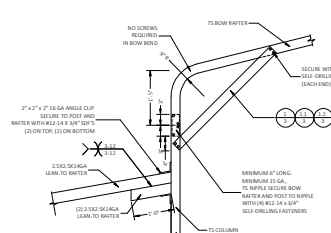
SIDE EXTENSION RAFTER/COLUMN DETAIL FOR EXTENSION RAFTER SPANS 12'-0" < W < 16'-0", IF THE KNEE BRACE ON THE OTHER END OF THE RAFTER IS PER DETAIL 1.2/3 FOR EXTENSION RAFTER SPANS 13'-0" < W < 18'-0", IF THE KNEE BRACE ON THE OTHER END OF THE RAFTER IS PER DETAIL 1.2/3 FOR EXTENSION RAFTER SPANS 15'-0" < W < 19'-0", IF THE KNEE BRACE ON THE OTHER END OF THE RAFTER IS PER DETAIL 1.3/3 SCALE: NTS
