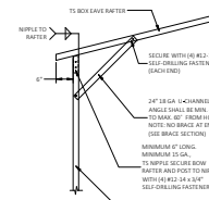
1.2 BOX EAVE RAFTER COLUMN CONNECTION DETAIL FOR HEIGHTS 12'-0" < W <= 30' - 0" MAXIMUM RAFTER SPAN SCALE: NTS
