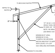
1 BOX EAVE RAFTER COLUMN CONNECTION DETAIL FOR HEIGHTS 12'-0" < W <= 30' - 0" MAXIMUM RAFTER SPAN SCALE: NTS
