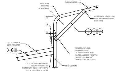
SIDE EXTENSION RAFTER/COLUMN DETAIL FOR EXTENSION RAFTER SPANS 16'-0" \times W \times 24'-0", IF THE KNEE BRACE ON THE OTHER END OF THE RAFTER IS PER DETAIL 1.2/3 FOR EXTENSION RAFTER SPANS 18'-0" \times W \times 24'-0", IF THE KNEE BRACE ON THE OTHER END OF THE RAFTER IS PER DETAIL 1.2/3 FOR EXTENSION RAFTER SPANS 19'-0" \times W \times 24'-0", IF THE KNEE BRACE ON THE OTHER END OF THE RAFTER IS PER DETAIL 1.2/3 SCALE: NTS
