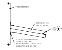
LEAN-TO RAFTER TO RAFTER COLUMN CONNECTION DETAIL FOR LEAN-TO RAFTER SPANS 16'-0" < W < 24'-0", IF THE KNEE BRACE ON THE OTHER END OF THE RAFTER IS PER DETAIL 1.2/2 OR 1.2/3, FOR LEAN-TO RAFTER SPANS 18'-0" < W < 24'-0", IF THE KNEE BRACE ON THE OTHER END OF THE RAFTER IS PER DETAIL 1.1/2 OR 1.1/3, FOR LEAN-TO RAFTER SPANS 19'-0" < W < 24'-0", IF THE KNEE BRACE ON THE OTHER END OF THE RAFTER IS PER DETAIL 1/2 OR 1/3. SCALE: NTS
