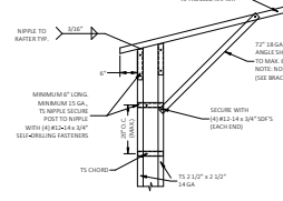
1B BOX EAVE RAFTER COLUMN CONNECTION DETAIL FOR HEIGHTS 12'-0" < W <= 30' - 0" MAXIMUM RAFTER SPAN SCALE: NTS
