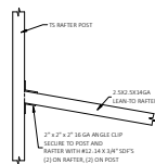
LEAN-TO RAFTER TO RAFTER COLUMN CONNECTION DETAIL FOR LEAN-TO RAFTER SPANS W \leq 12'-0" , IF THE KNEE BRACE ON THE OTHER END OF THE RAFTER IS PER DETAIL 1/2/ OR 1/3/ FOR LEAN-TO RAFTER SPANS W = 13'-0" , IF THE KNEE BRACE ON THE OTHER END OF THE RAFTER IS PER DETAIL 1/2/ OR 1/3/ FOR LEAN-TO RAFTER SPANS W > 15'-0" , IF THE KNEE BRACE ON THE OTHER END OF THE RAFTER IS PER DETAIL 1/2/ OR 1/3. SEE F.N.TS.
