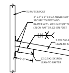
LEAN-TO RAFTER TO RAFTER COLUMN CONNECTION DETAIL FOR LEAN-TO RAFTER SPANS 12'-0" < W < 16'-0" , IF THE KNEE BRACE ON THE OTHER END OF THE RAFTER IS PER DETAIL 1/2 OR 1/2.3, FOR LEAN-TO RAFTER SPANS 13'-0" < W < 18'-0" , IF THE KNEE BRACE ON THE OTHER END OF THE RAFTER IS PER DETAIL 1/2 OR 1/2.3, FOR LEAN-TO RAFTER SPANS 15'-0" < W < 19'-0" , IF THE KNEE BRACE ON THE OTHER END OF THE RAFTER IS PER DETAIL 1/2 OR 1/3. SCALE: NTS
