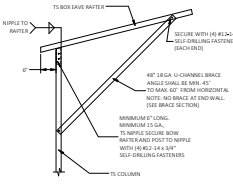
1.1 BOX EAVE RAFTER COLUMN CONNECTION DETAIL FOR HEIGHTS 12'-0" < W <= 30' - 0" MAXIMUM RAFTER SPAN SCALE: NTS
