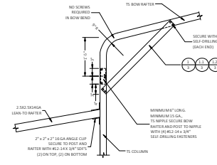
SIDE EXTENSION RAFTER/COLUMN DETAIL FOR EXTENSION RAFTER SPANS W' < 12'-0" , IF THE KNEE BRACE ON THE OTHER END OF THE RAFTER IS PER DETAIL 1.2/3 FOR EXTENSION RAFTER SPANS W' < 13'-0" , IF THE KNEE BRACE ON THE OTHER END OF THE RAFTER IS PER DETAIL 1.3/3 FOR EXTENSION RAFTER SPANS W' < 15'-0" , IF THE KNEE BRACE ON THE OTHER END OF THE RAFTER IS PER DETAIL 1.3/3 SC-616-MTS
