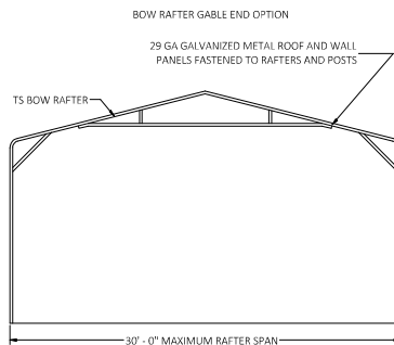
TYPICAL RAFTER/POST FRAME SECTION EXTRA SIDE PANELS
