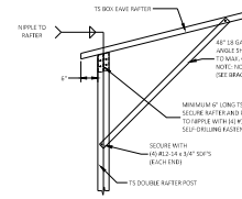
1A BOX EAVE RAFTER COLUMN CONNECTION DETAIL FOR HEIGHTS 18'-0" < TO 19'-0" SCALE: NTS
