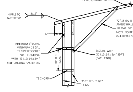
1B BOX EAVE RAFTER COLUMN CONNECTION DETAIL FOR HEIGHTS 19'-0" < TO 20'-0" SCALE: NTS
