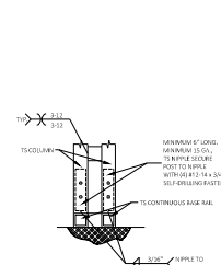
2B RAFTER POST/BASE RAIL CONNECTION DETAIL SCALE: NTS
