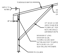
1 BOX EAVE RAFTER COLUMN CONNECTION DETAIL FOR HEIGHTS 12'-0" < TO 13'-0" SCALE: NTS
