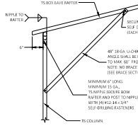
1.1 BOX EAVE RAFTER COLUMN CONNECTION DETAIL FOR HEIGHTS 13'-0" < TO 15'-0" SCALE: NTS
