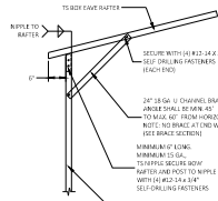
1.2 BOX EAVE RAFTER COLUMN CONNECTION DETAIL FOR HEIGHTS 15'-0" < TO 17'-0" SCALE: NTS
