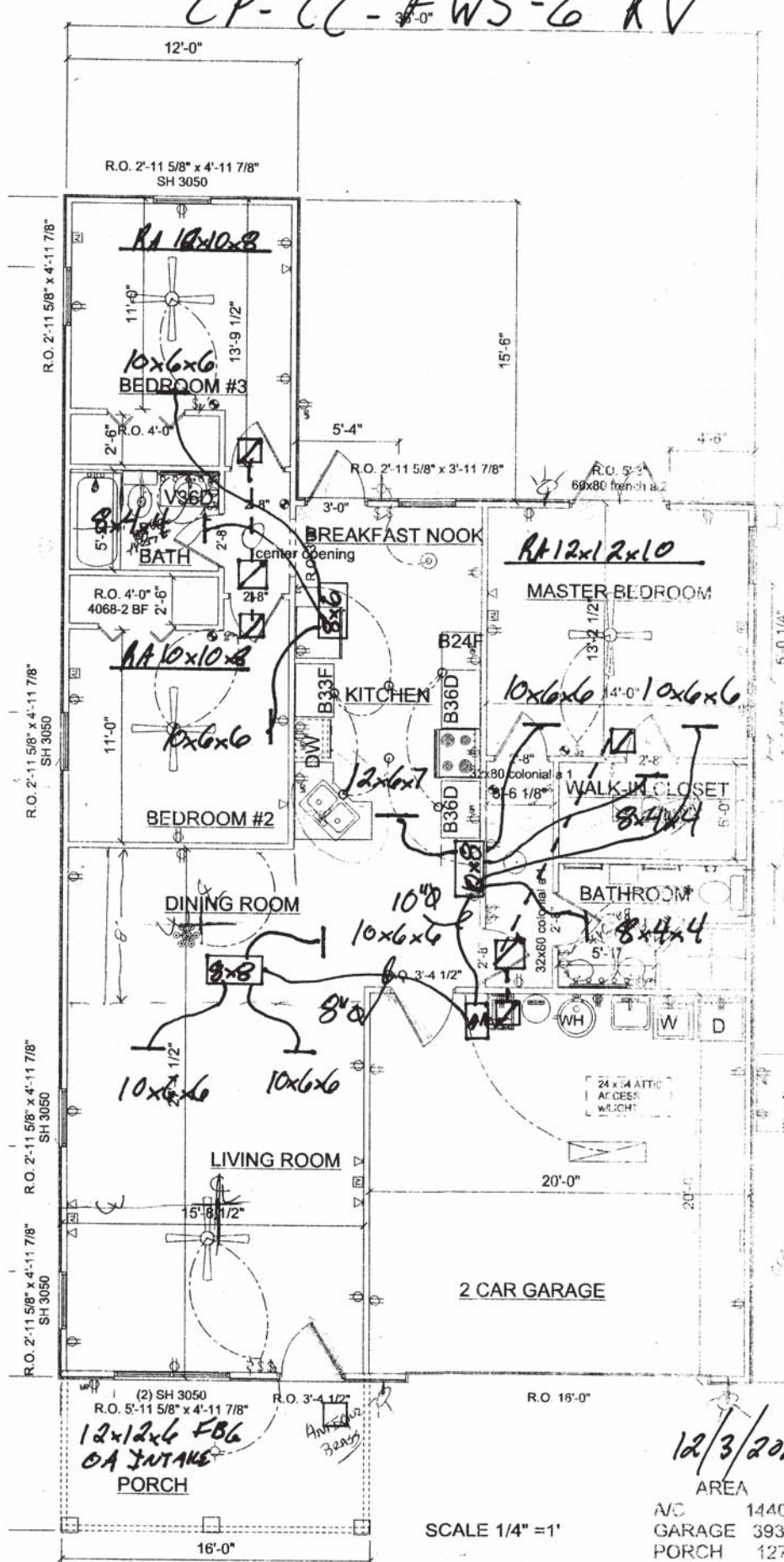
FLOOR PLAN
