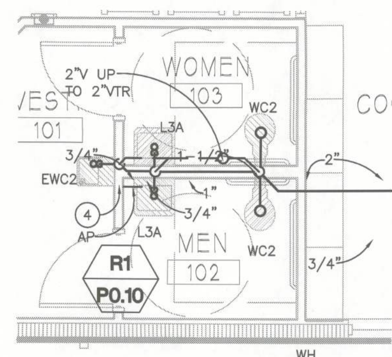
PARTIAL FLOOR PLAN - SANITARY WASTE AND VENT PIPING SCALE: 1/4" = 1'-0"
