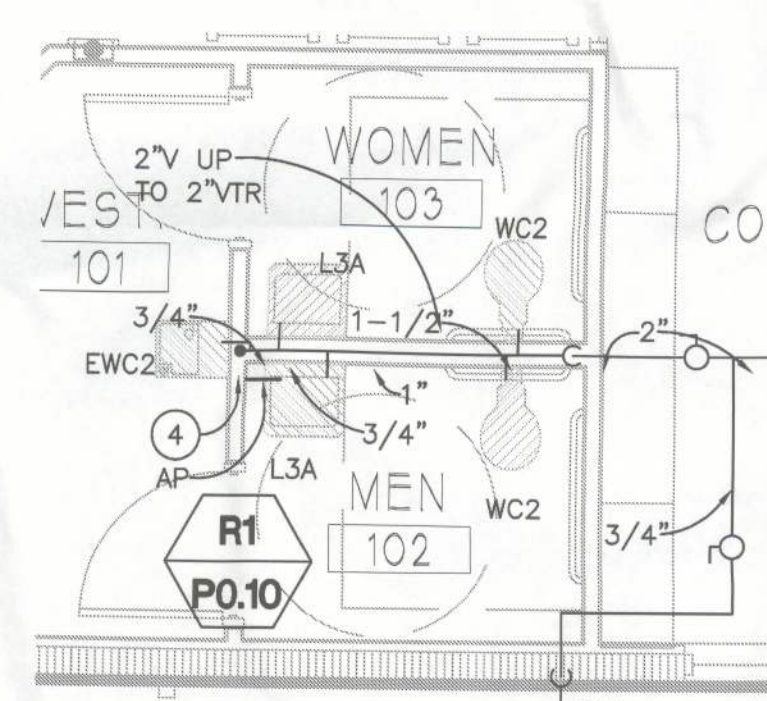
PARTIAL FLOOR PLAN - WATER PIPING SCALE: 1/4" = 1'-0"
