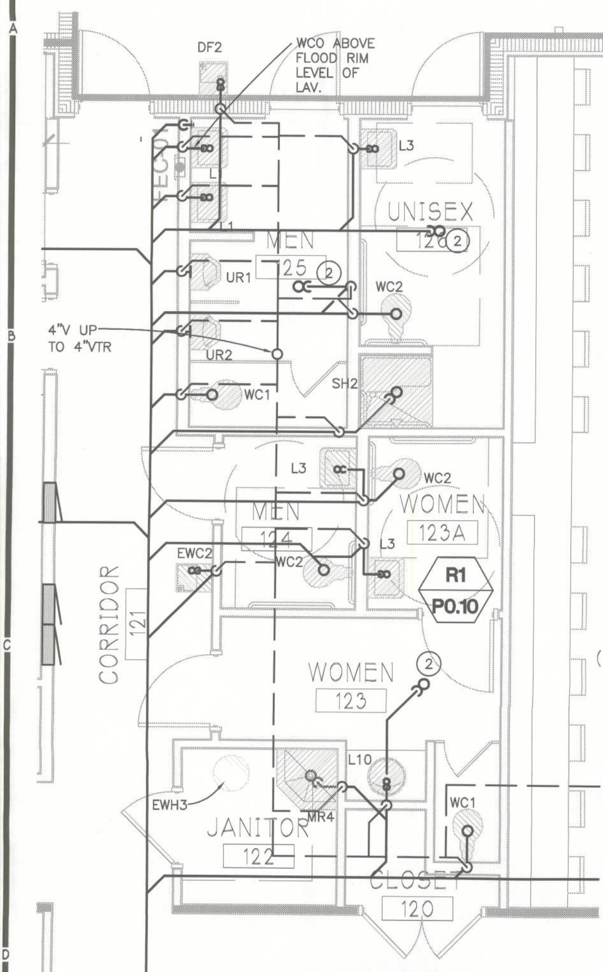
PARTIAL FLOOR PLAN - SANITARY WASTE AND VENT PIPING SCALE: 1/4" = 1'-0"
