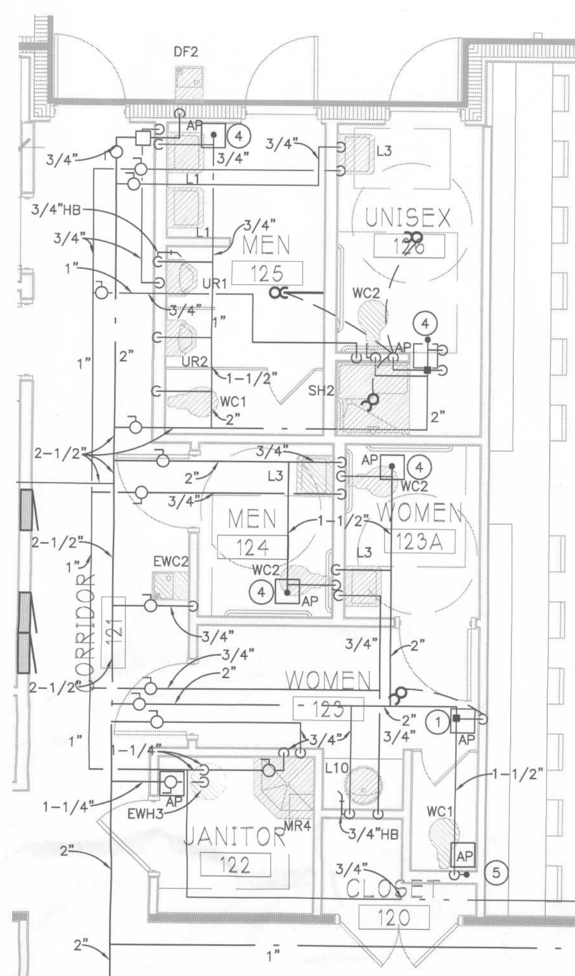
PARTIAL FLOOR PLAN - WATER PIPING SCALE: 1/4" = 1'-0"
