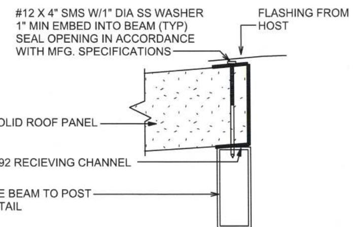
SOLID ROOF PANEL ATTACHMENT TO 4TH WALL NTS
