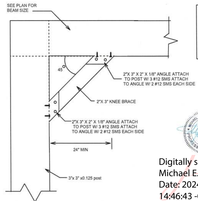
KNEE BRACE COLUMN TO BEAM
