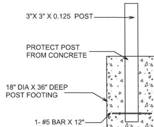
POST FOOTING 3"X 3" X 0.125
