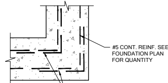
FM19 TYP. CORNER BAR DETAIL SCALE: 3/4" = 1'-0" @ 22x34 SCALE: 3/8" = 1'-0" @ 11x17
