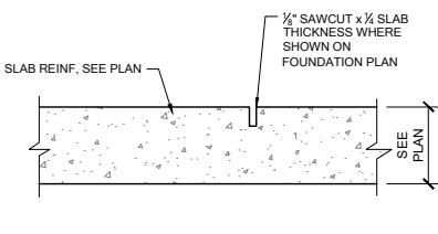
FM20 CONTROL JOINT SCALE: 3/4" = 1'-0" @ 22x34 SCALE: 3/8" = 1'-0" @ 11x17
