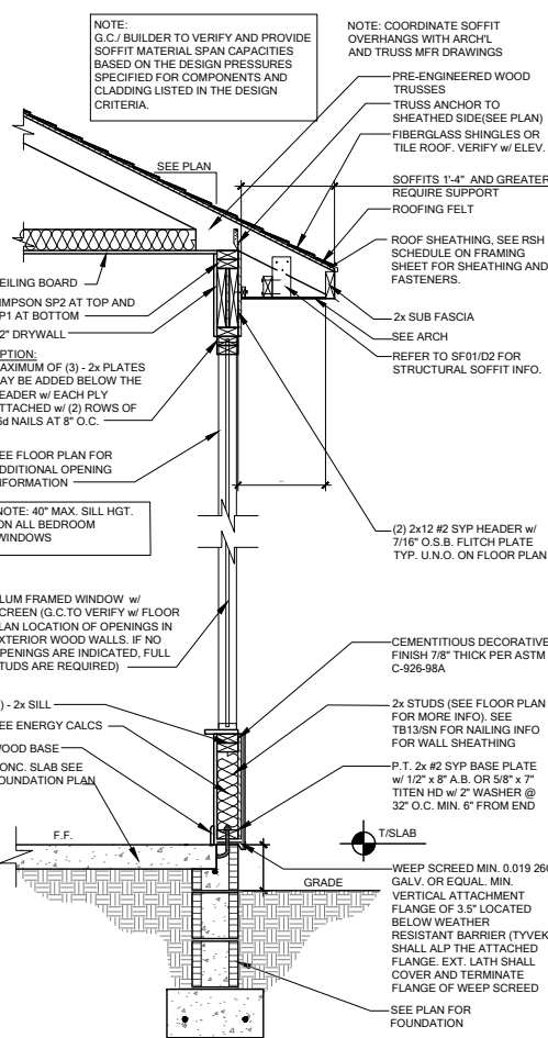
WS02 TYP. WALL SECTION SCALE: 3/4" = 1'-0" @ 22x34 SCALE: 3/8" = 1'-0" @ 11x17
