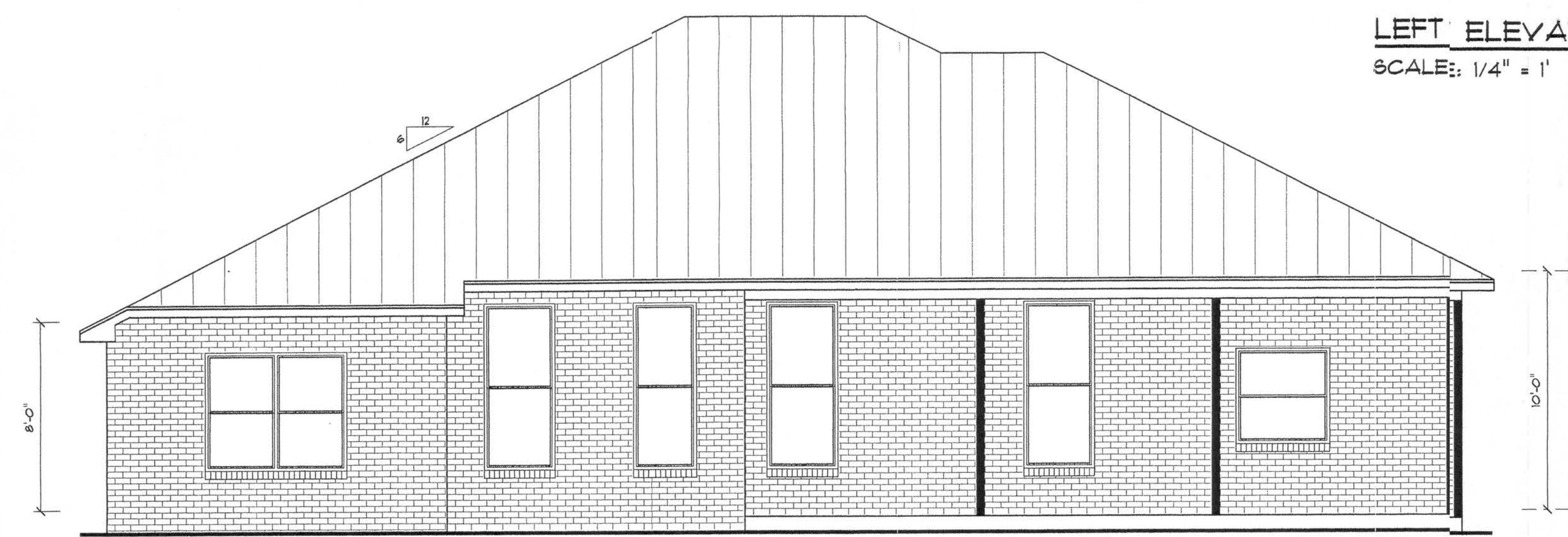
REAR ELEVATION SCALE: 1/4" = 1'
