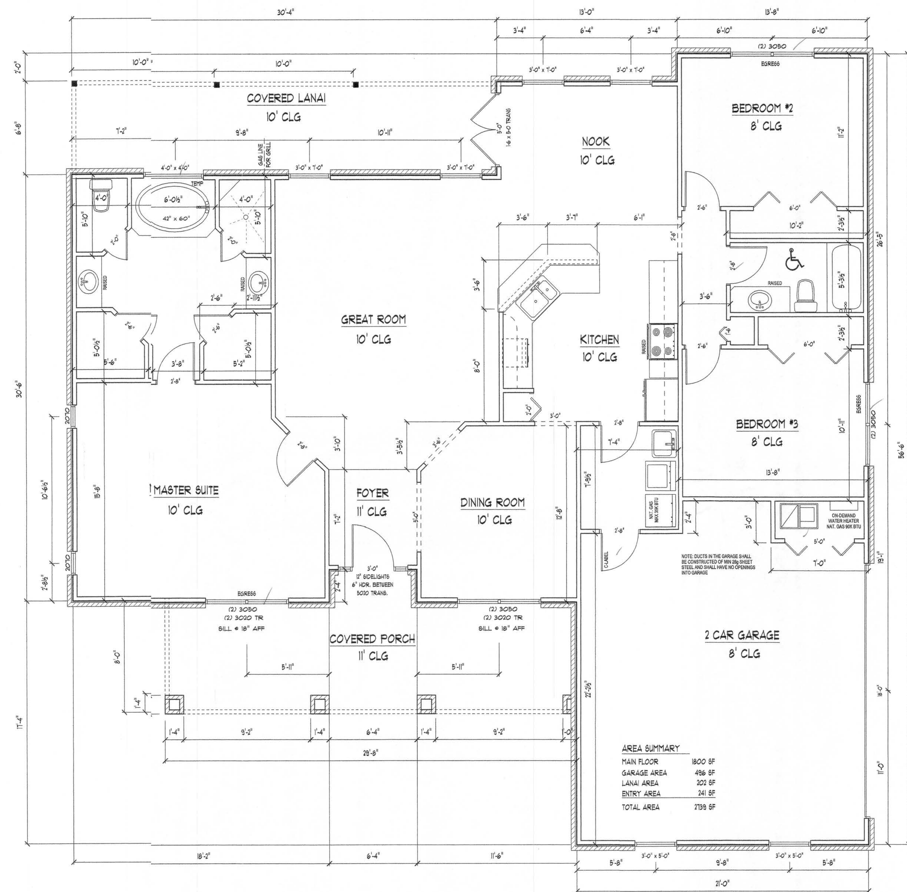
FLOOR PLAN SCALE: 1/4" = 1'
