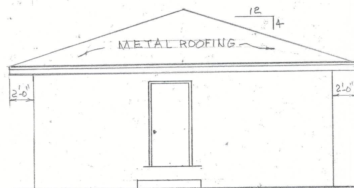
RIGHT SIDE ELEVATION SCALE: 1/4" = 1'-0"
