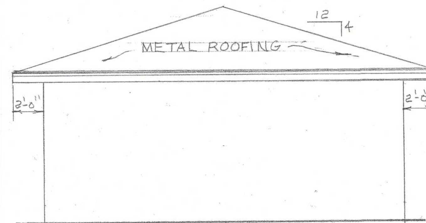
LEFT SIDE ELEVATION SCALE: 1/4" = 1'-0"
