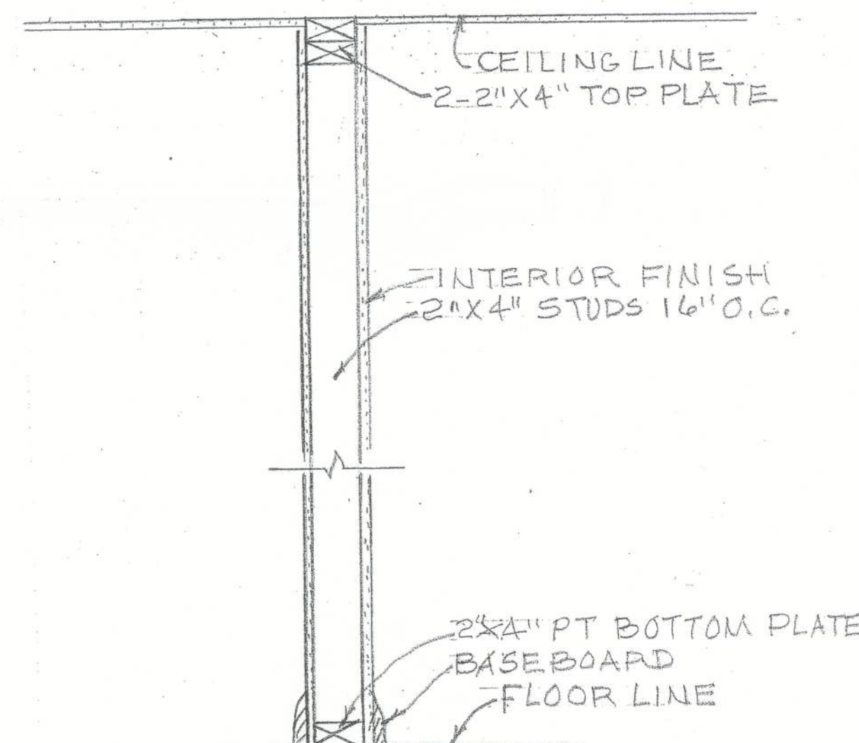
INTERIOR WALL SECTION SCALE: 1" = 1'-0"
