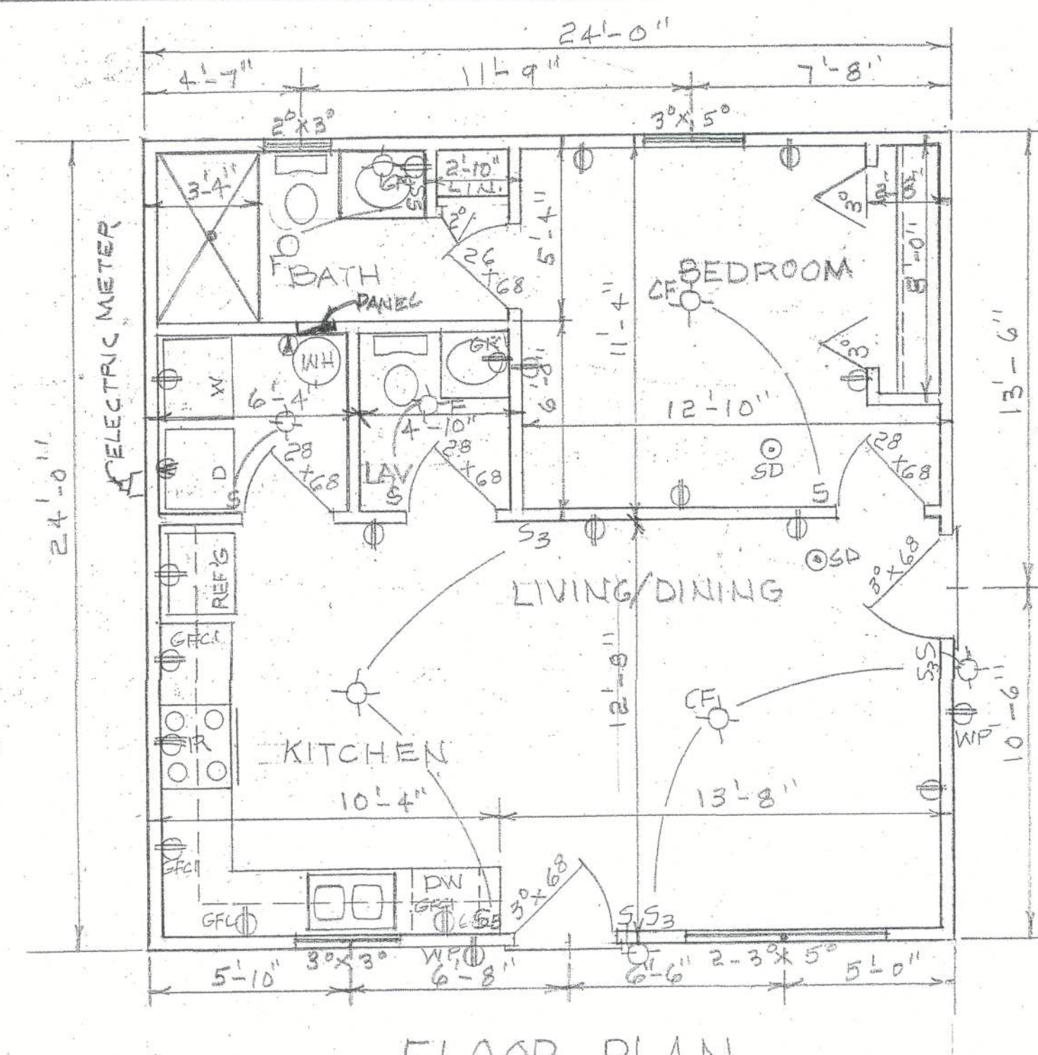
FLOOR PLAN SCALE: 1/4" = 1'-0" 576 SQ. FT.
