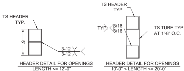
SIDE WALL OPTION HEADER SCALE: NTS
