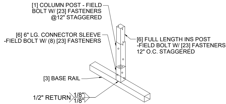
3. BASE DETAIL
