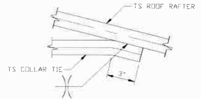
COLLAR TIE CONNECTION DETAIL
