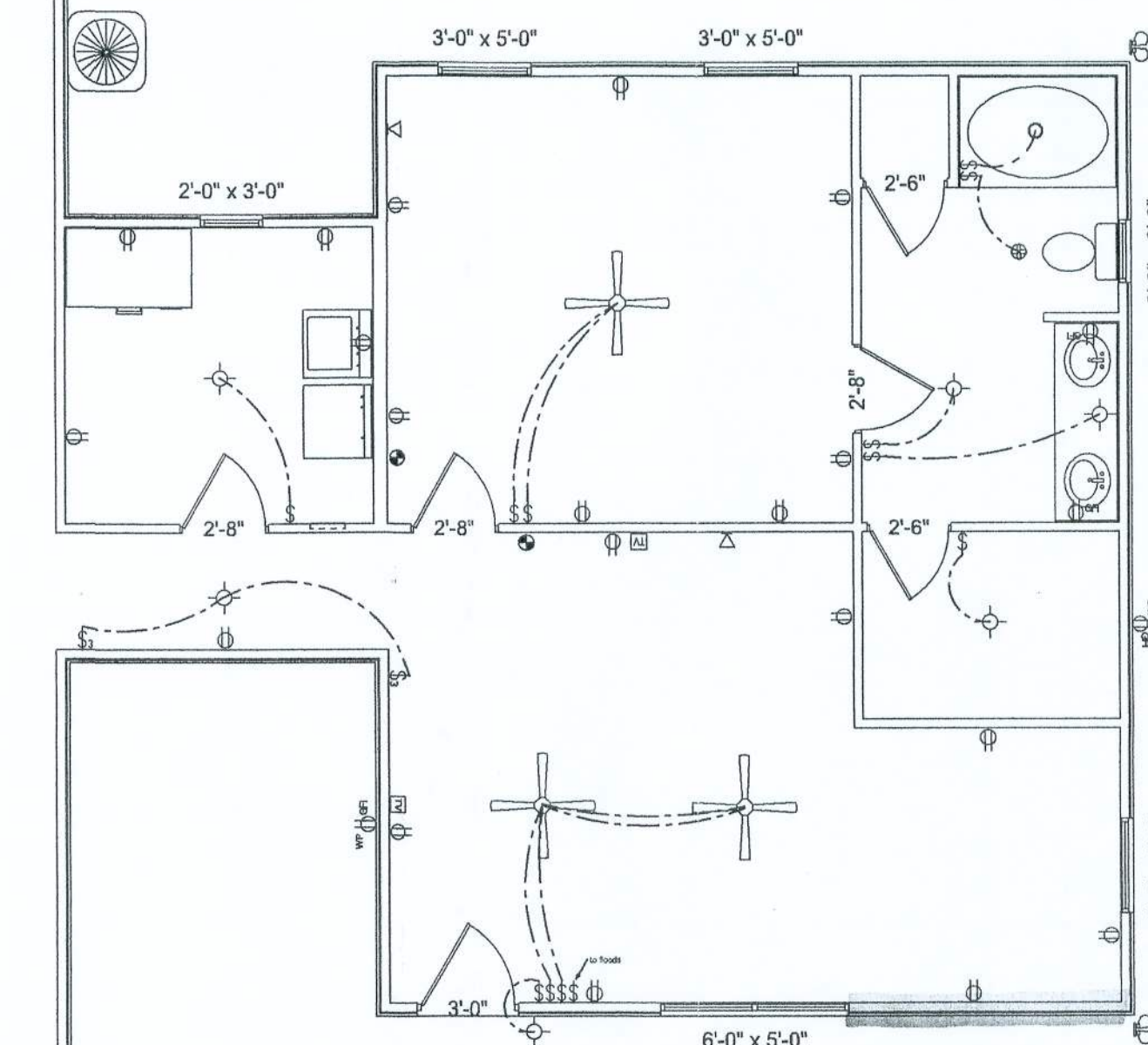
ELECTRICAL PLAN
