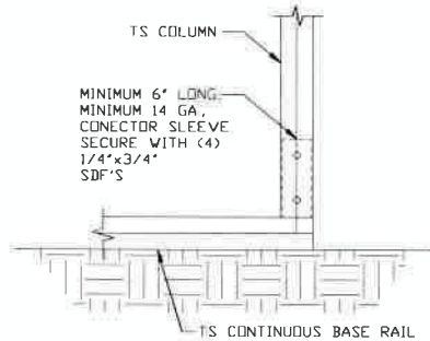
13 COLUMN/BASE RAIL CONNECTION DETAIL
