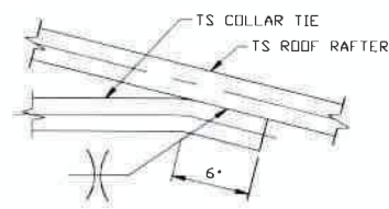
12 COLLAR TIE CONNECTION DETAIL
