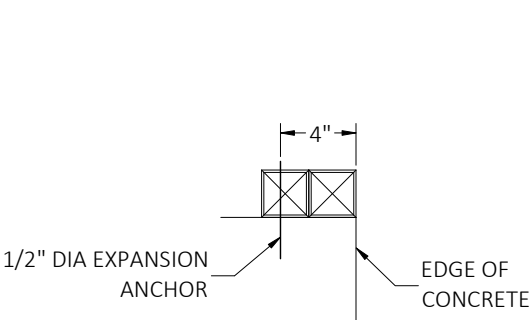
SECTION (OPTION-1)
