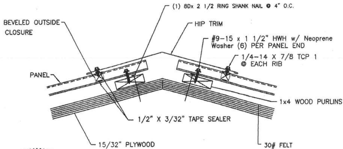
TYPICAL DETAILS HIP
