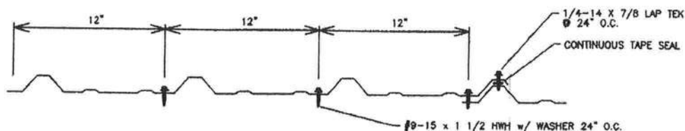
TYPE 1 FASTENER PATTERN
