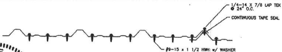
FASTENER PATTERN AT EAVE & VALLEY
