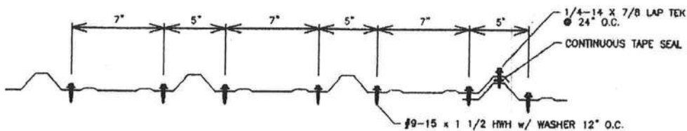
TYPE 2 FASTENER PATTERN
