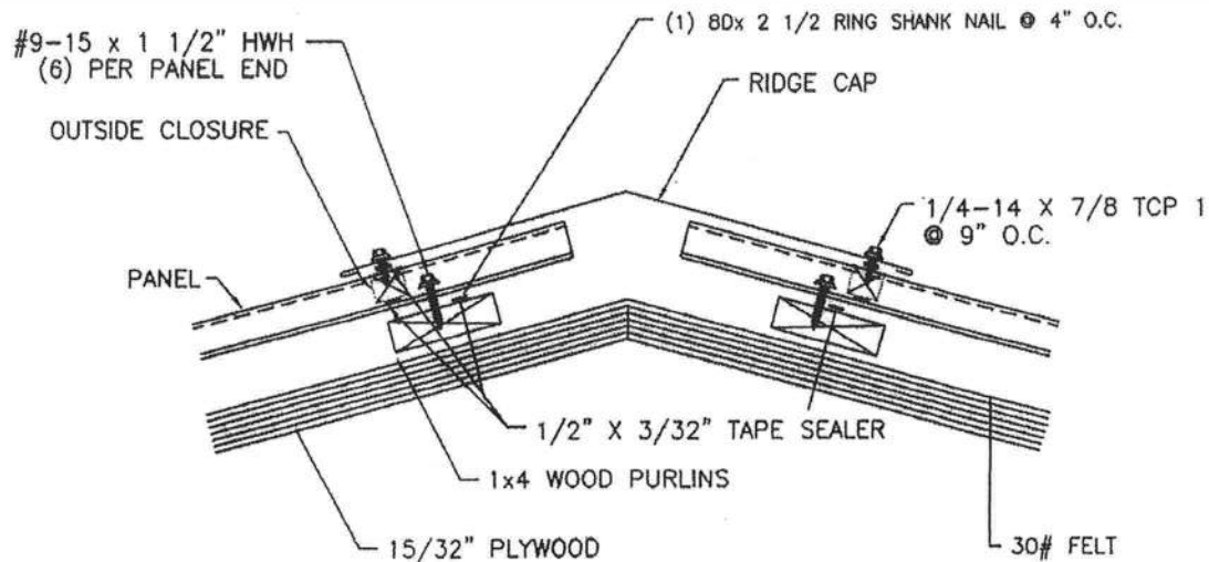
TYPICAL DETAILS RIDGE
