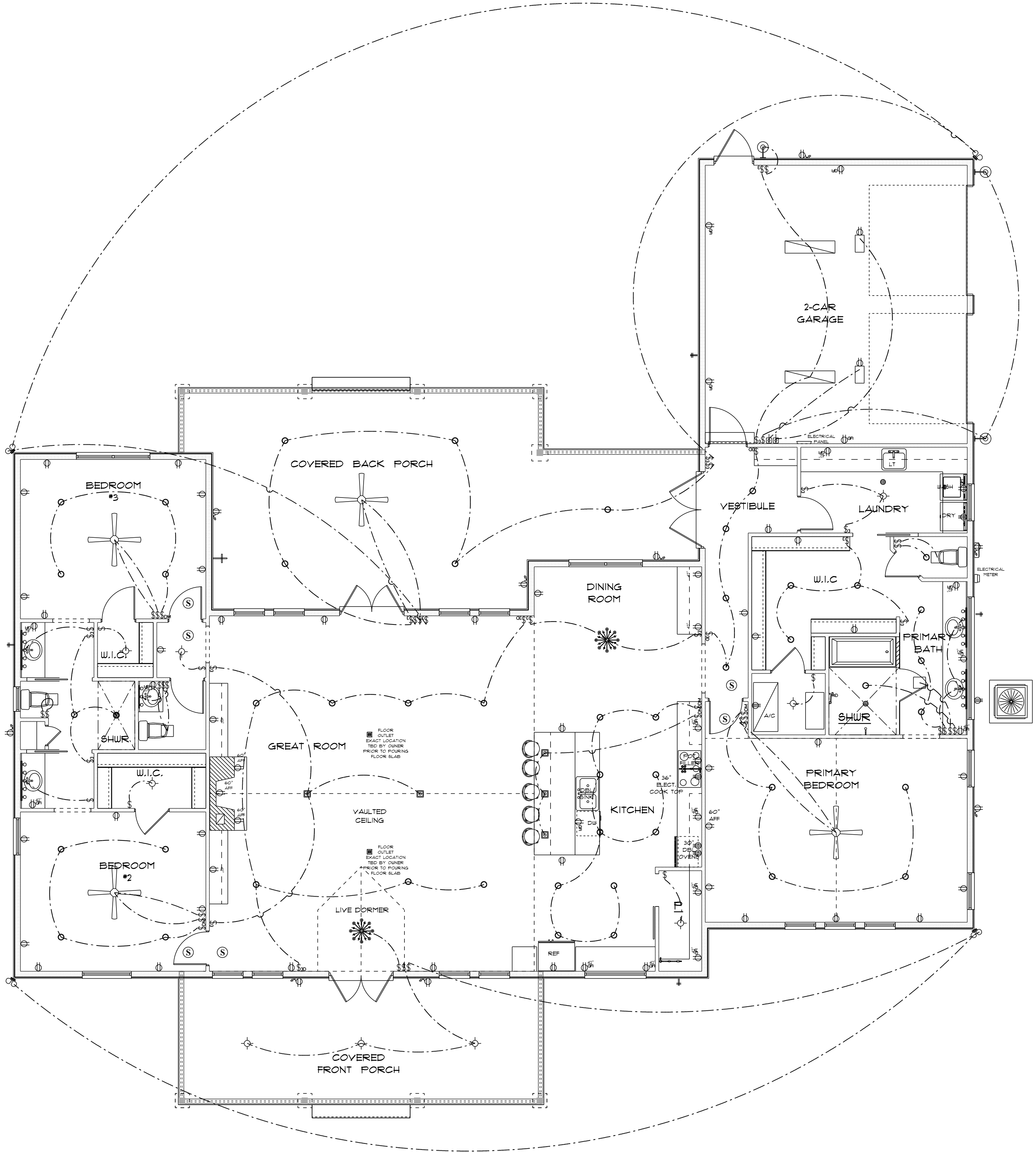
* ELECTRICAL PLAN *
