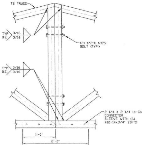
13 SPLICE CONNECTION DETAIL
