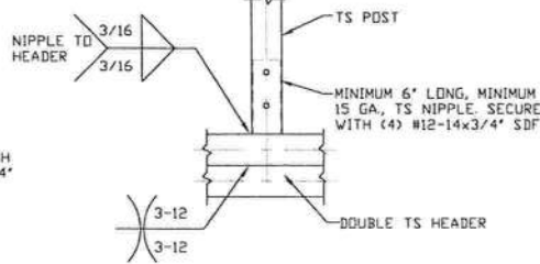
11 POST/DOUBLE HEADER CONNECTION DETAIL
