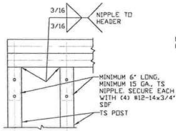
10 DOUBLE HEADER/POST CONNECTION DETAIL
