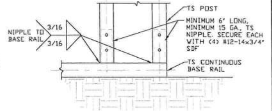
12 POST/BASE RAIL CONNECTION DETAIL
