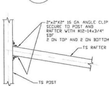
LEAN-TO RAFTER TO RAFTER COLUMN CONNECTION DETAIL FOR RAFTER SPANS 12'-0"
