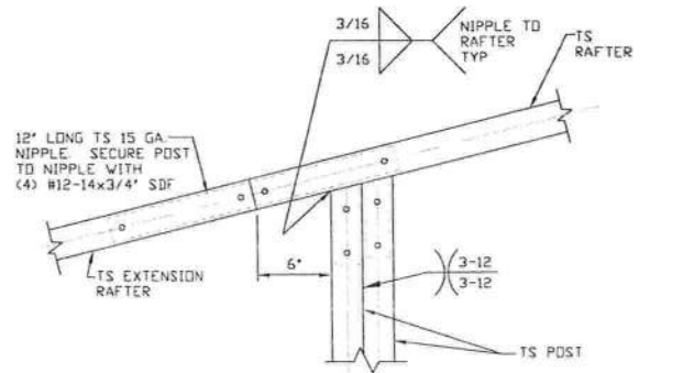
SIDE EXTENSION RAFTER/COLUMN DETAIL FOR RAFTER SPANS < 12'-0"
