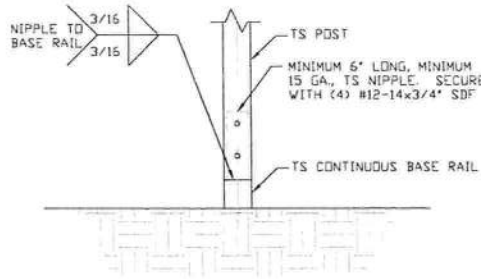
LEAN-TO POST CONNECTION DETAIL
