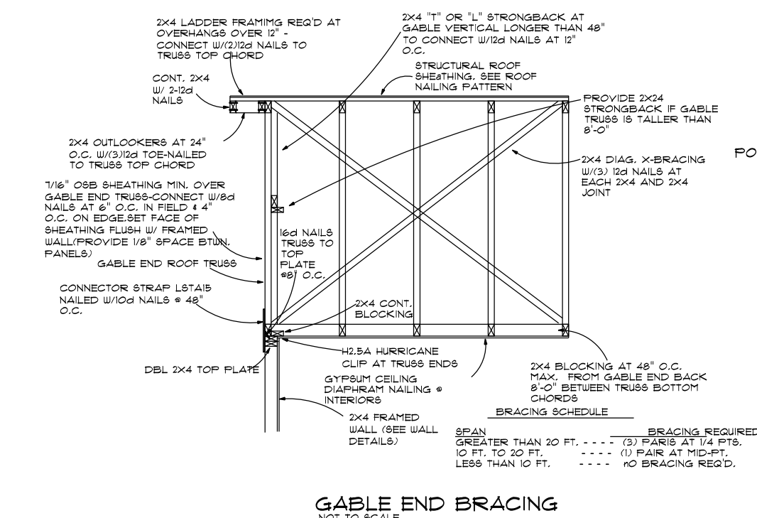
GABLE END BRACING NOT TO SCALE
