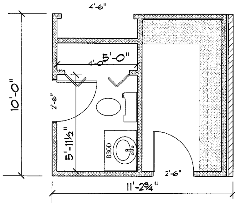
Existing Room Layout
