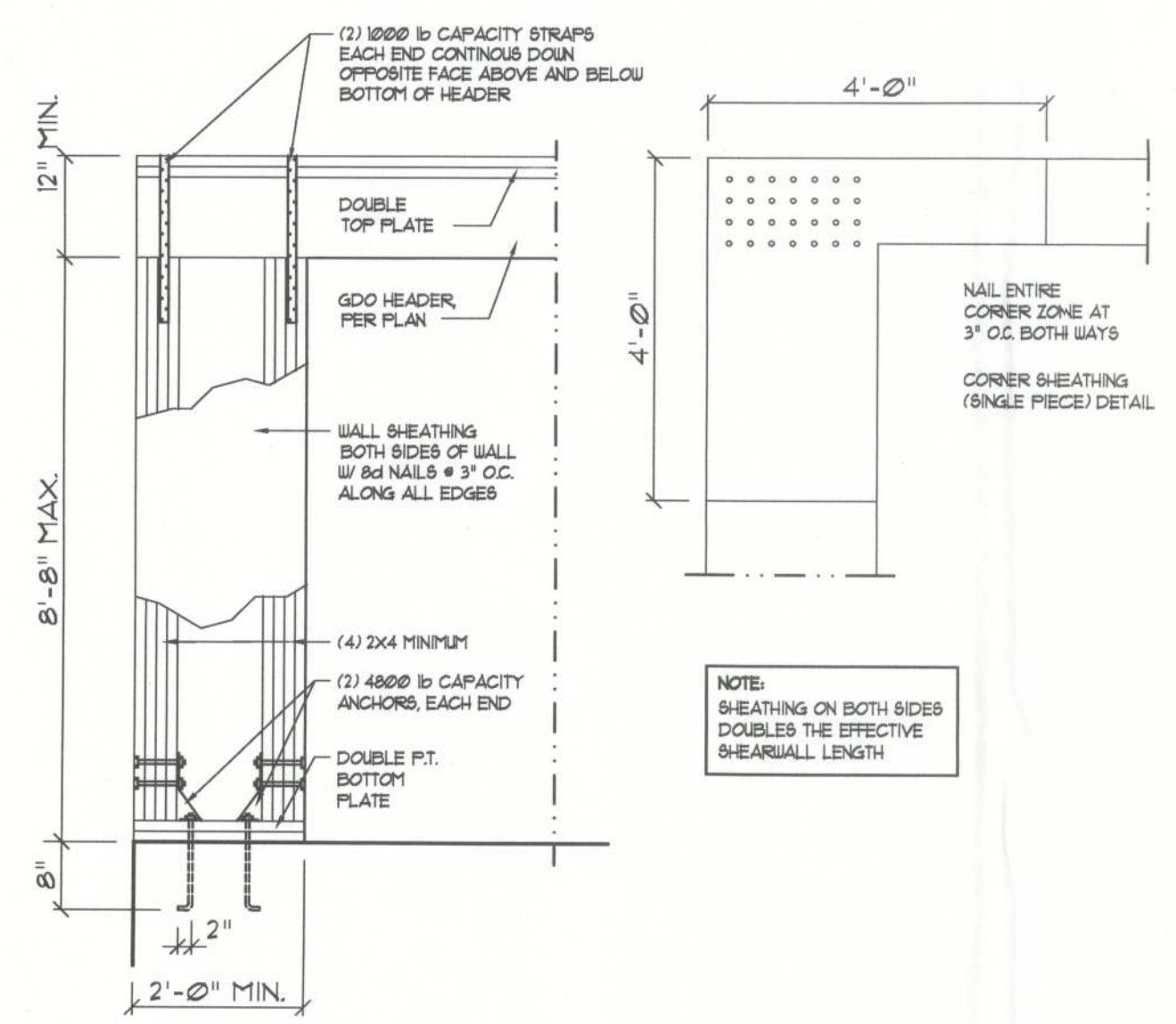
Garage End Wall DETAILS B SCALE: 1/2" = 1'-0"
