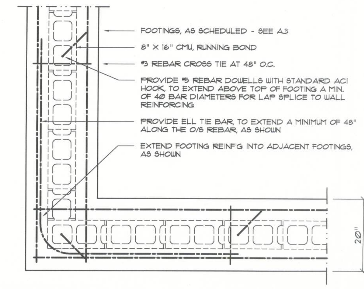
Wall/End Reinf'g DETAIL A SCALE: 3/4" = 1'-0"
