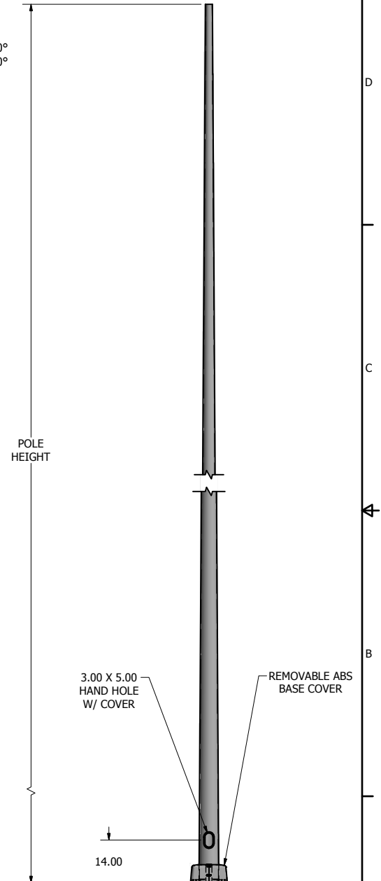
POLE DETAIL
