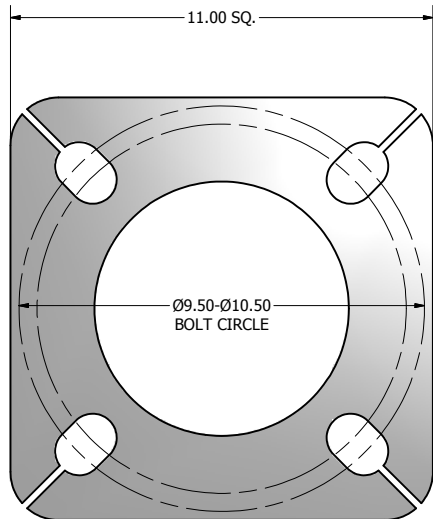
11.00 X 11.00 X 1.00 THK. BASE PLATE
