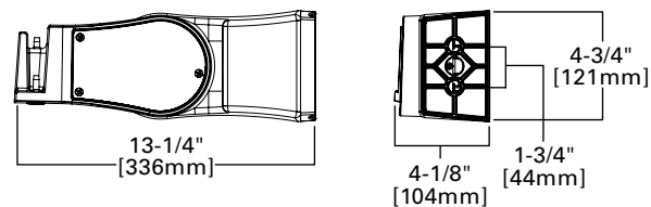
Adjustable Wall Mount (PRV-XL)
