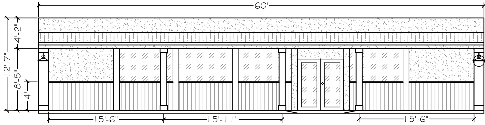
FRONT ELEVATION - OFFICE SCALE: 1/8" = 1'
