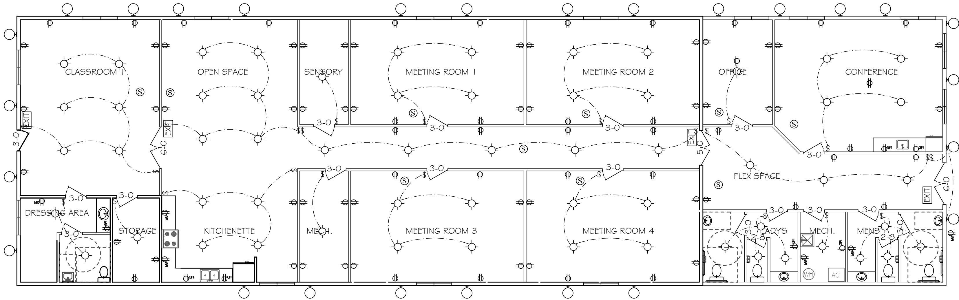
ELECTRIC PLAN SCALE: 1/8" = 1'
