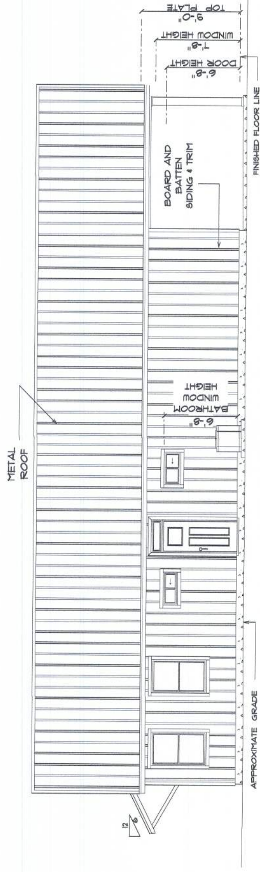
• LEFT ELEVATION • SCALE : 1/4" = 1'-0"
