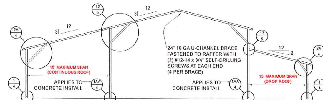
TYPICAL LEAN-TO OPTIONS FRAMING PLAN (BOTH OPTIONS SHOWN) NOT TO SCALE
