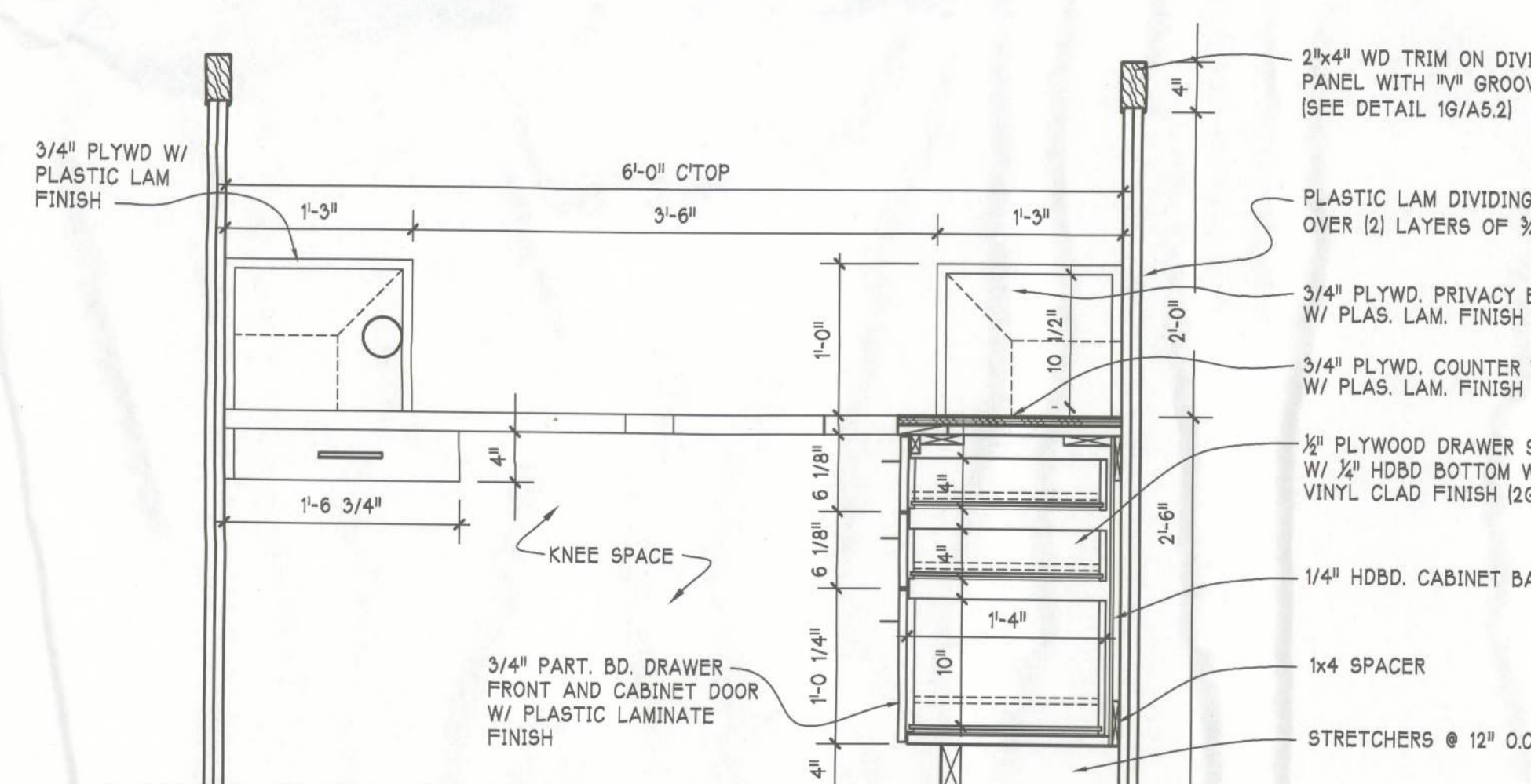
3G A5.2 SECTION THRU CUSTOMER SERVICE STATION SCALE: 1" = 1'-0"
