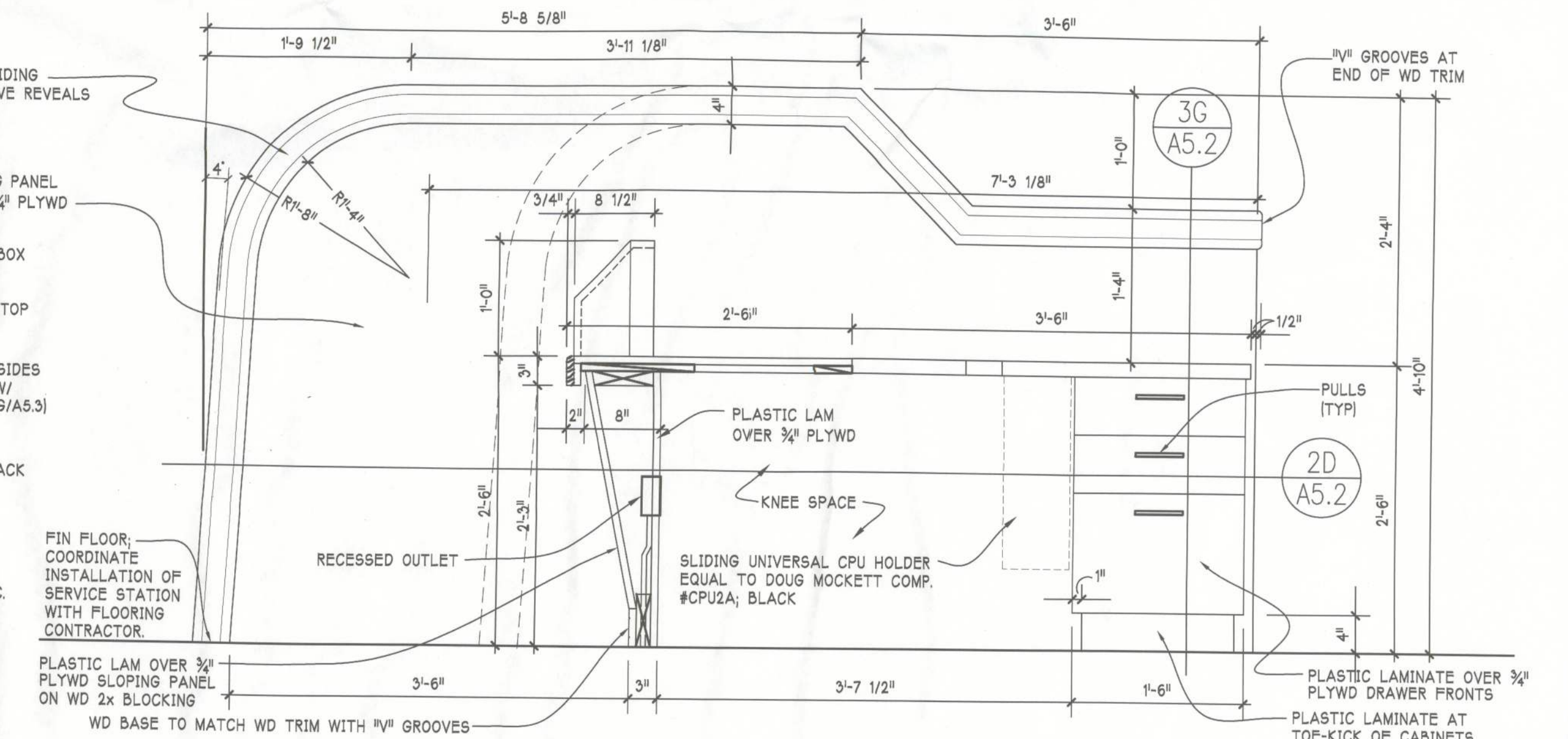
6G A5.2 SECTION THRU CUSTOMER SERVICE STATION SCALE: 1" = 1'-0"
