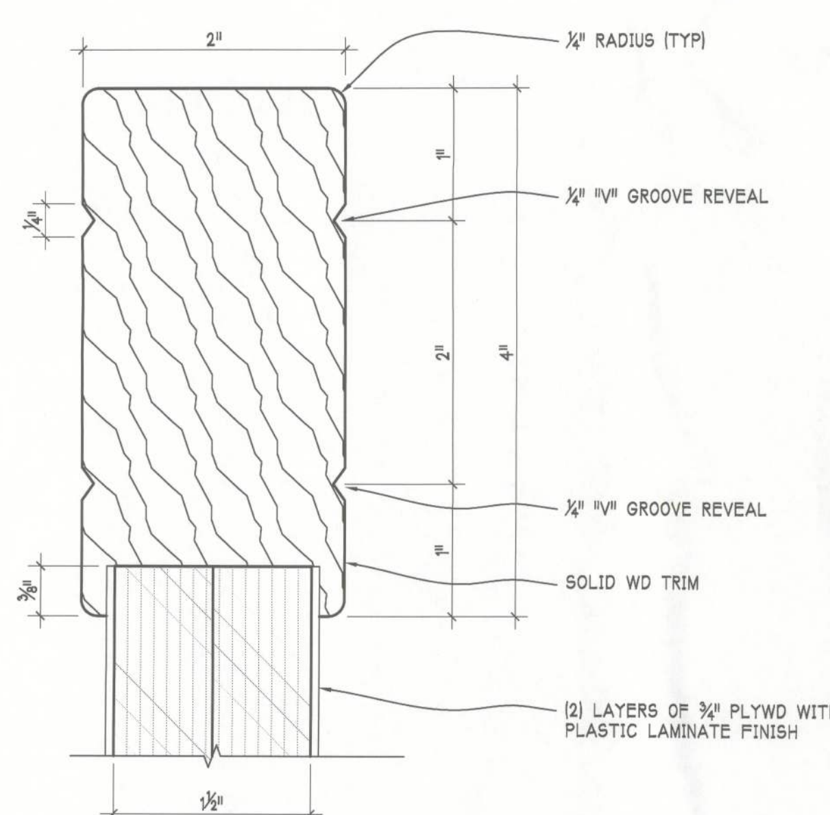
1G A5.2 DIVIDER PANEL WD TRIM DETAIL FULL SCALE
