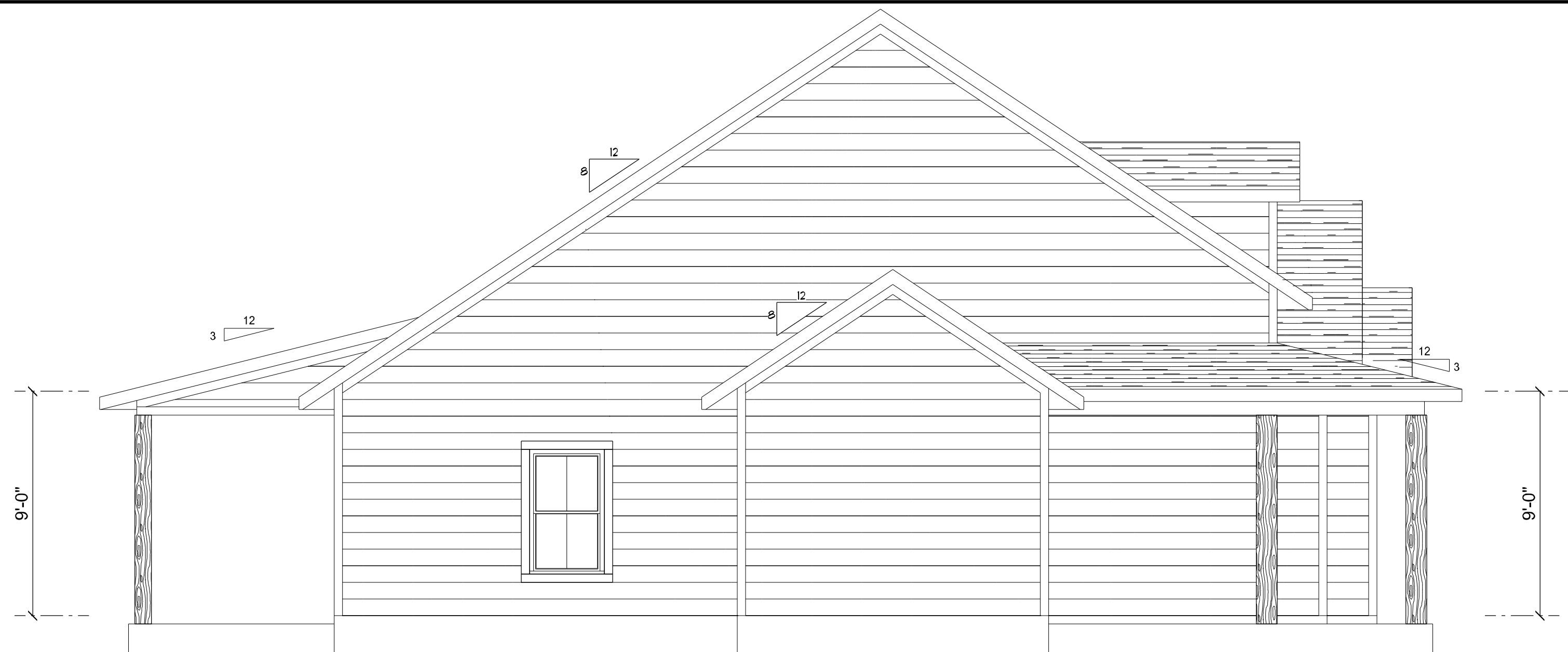
LEFT ELEVATION
