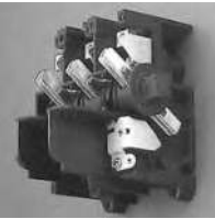
Visible Double-Break Rotary Blade Mechanism
