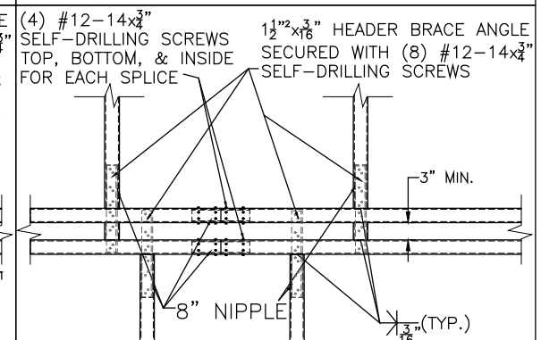
HEADER CONNECTION DETAIL OPTION 2
