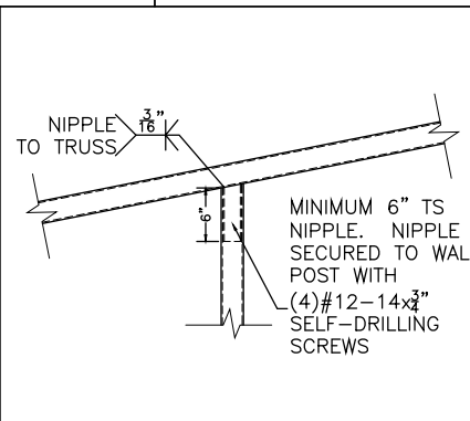
POST TO TRUSS CONNECTION
