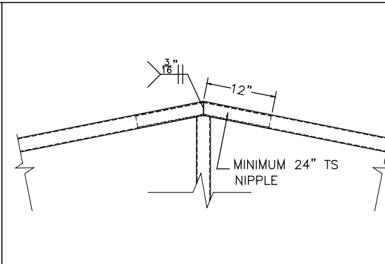
RAFTER CONNECTION DETAIL
