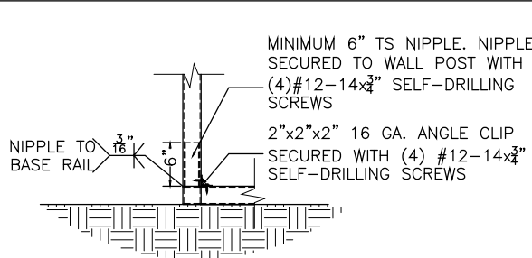
END POST TO BASE RAIL CONNECTION
