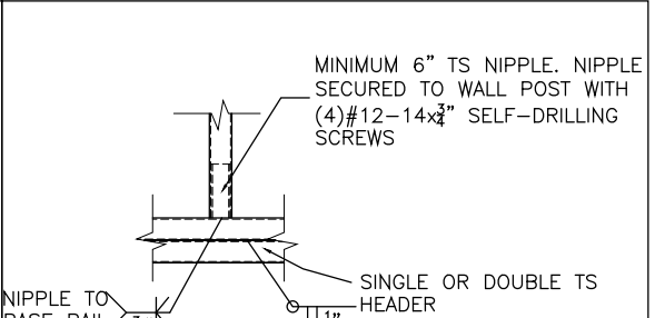
HEADER CONNECTION DETAIL OPTION 2
