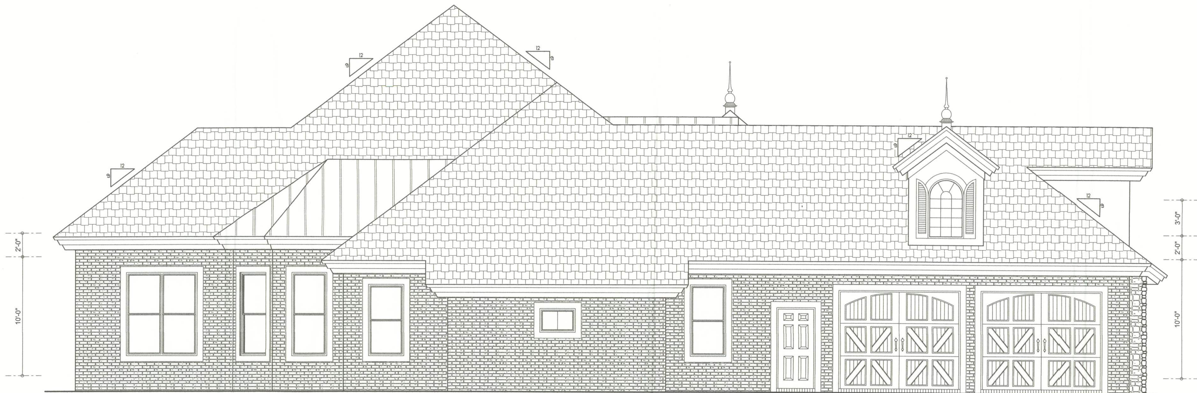
LEFT ELEVATION SCALE: 3/16" = 1'-0"
