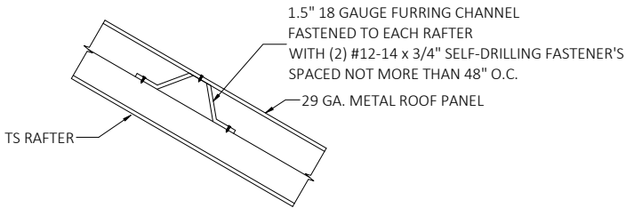
TS RAFTER ROOF PANEL ATTACHMENT SCALE: NTS
