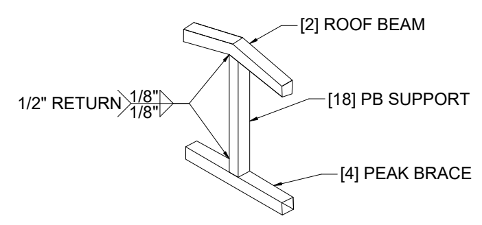
4. PB SUPPORT DETAIL
