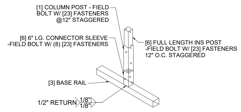
3. BASE DETAIL
