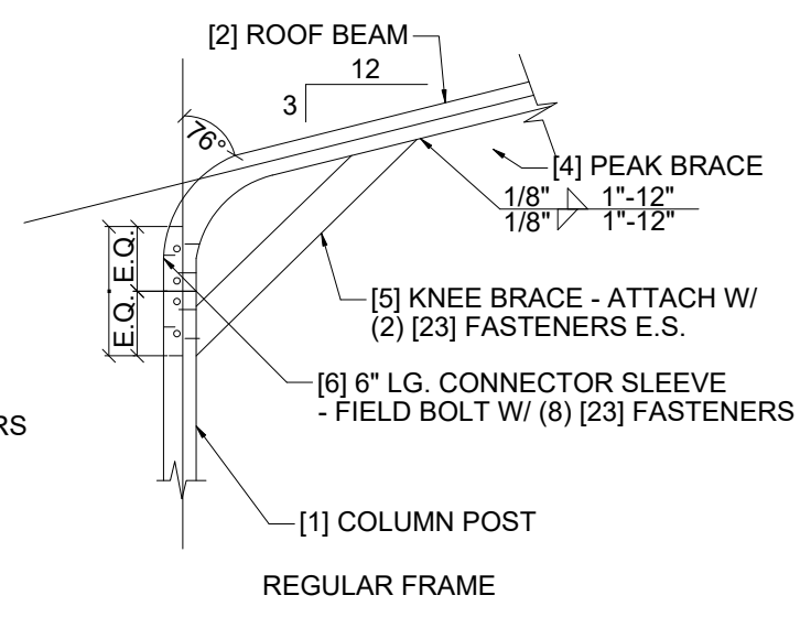
1. EAVE DETAIL OPTIONS
