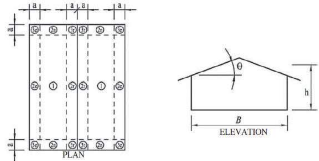
Figure 2: ASCE 7 Roof Zones for Gable Roofs 8^\circ \leq \Theta \leq 60^\circ
