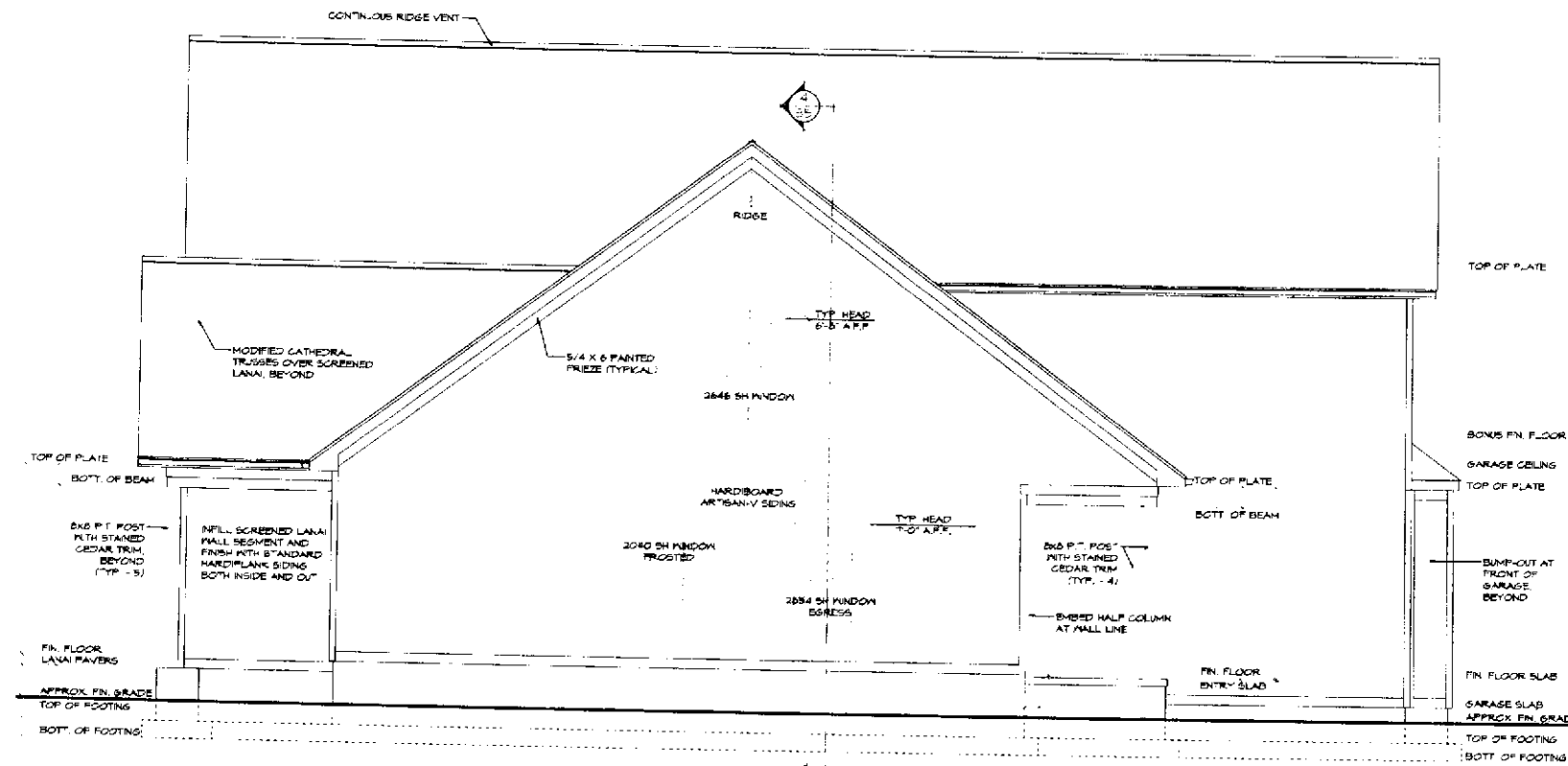
LEFT ELEVATION
