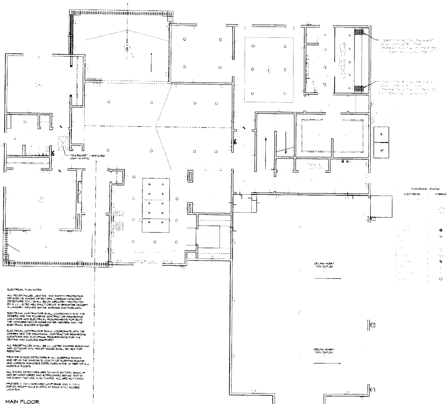
MAIN FLOOR ELECTRICAL PLAN SCALE: 1/4" = 1'-0"
