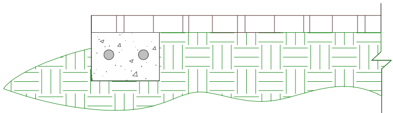
PAVERS W/ 12" X 12" FOOTER & (2) #5 THRU OUT
