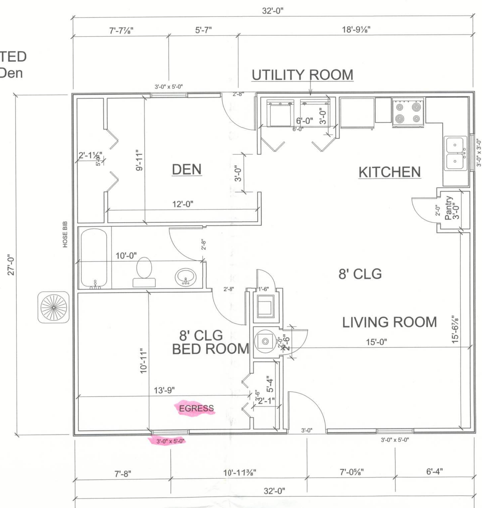
FLOOR PLAN
