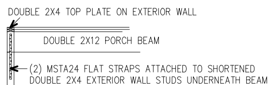
SIDE VIEW OF PORCH BEAM CONNECTION
