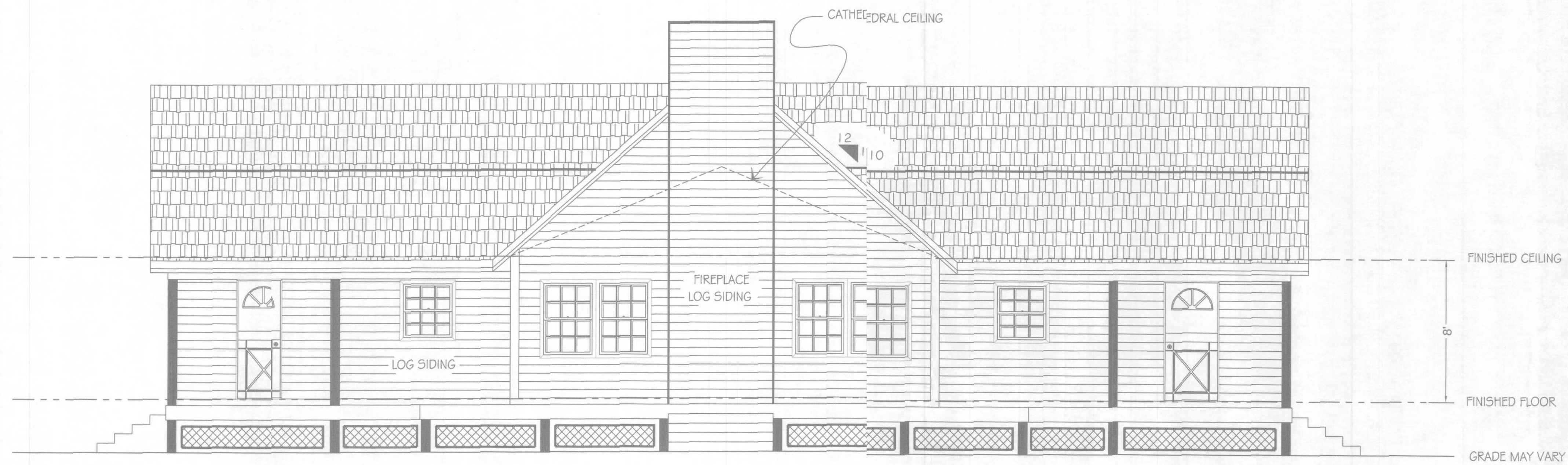
FRONT ELEVATION
