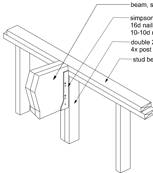
BEAM/WALL CONNECTION MAX. CAPACITY - 3640# DOWN; 1810# UPLIFT NOT TO SCALE
