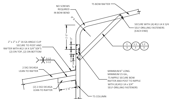
SIDE EXTENSION RAFTER/COLUMN DETAIL FOR EXTENSION RAFTER SPANS 12'-0" < W < 16'-0" , IF THE KNEE BRACE ON THE OTHER END OF THE RAFTER IS PER DETAIL 1.2/3. FOR EXTENSION RAFTER SPANS 13'-0" < W < 18'-0" , IF THE KNEE BRACE ON THE OTHER END OF THE RAFTER IS PER DETAIL 1.1/3. FOR EXTENSION RAFTER SPANS 15'-0" < W < 19'-0" , IF THE KNEE BRACE ON THE OTHER END OF THE RAFTER IS PER DETAIL 1/3. SCALE: NTS
