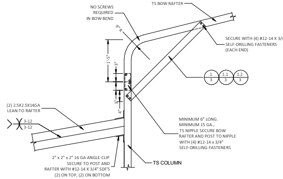
SIDE EXTENSION RAFTER/COLUMN DETAIL FOR EXTENSION RAFTER SPANS 16'-0" <W<=24'-0", IF THE KNEE BRACE ON THE OTHER END OF THE RAFTER IS PER DETAIL 1.2/3. FOR EXTENSION RAFTER SPANS 18'-0" <W<=24'-0", IF THE KNEE BRACE ON THE OTHER END OF THE RAFTER IS PER DETAIL 1.1/3. FOR EXTENSION RAFTER SPANS 19'-0" <W<=24'-0", IF THE KNEE BRACE ON THE OTHER END OF THE RAFTER IS PER DETAIL 1/3. SCALE: NTS
