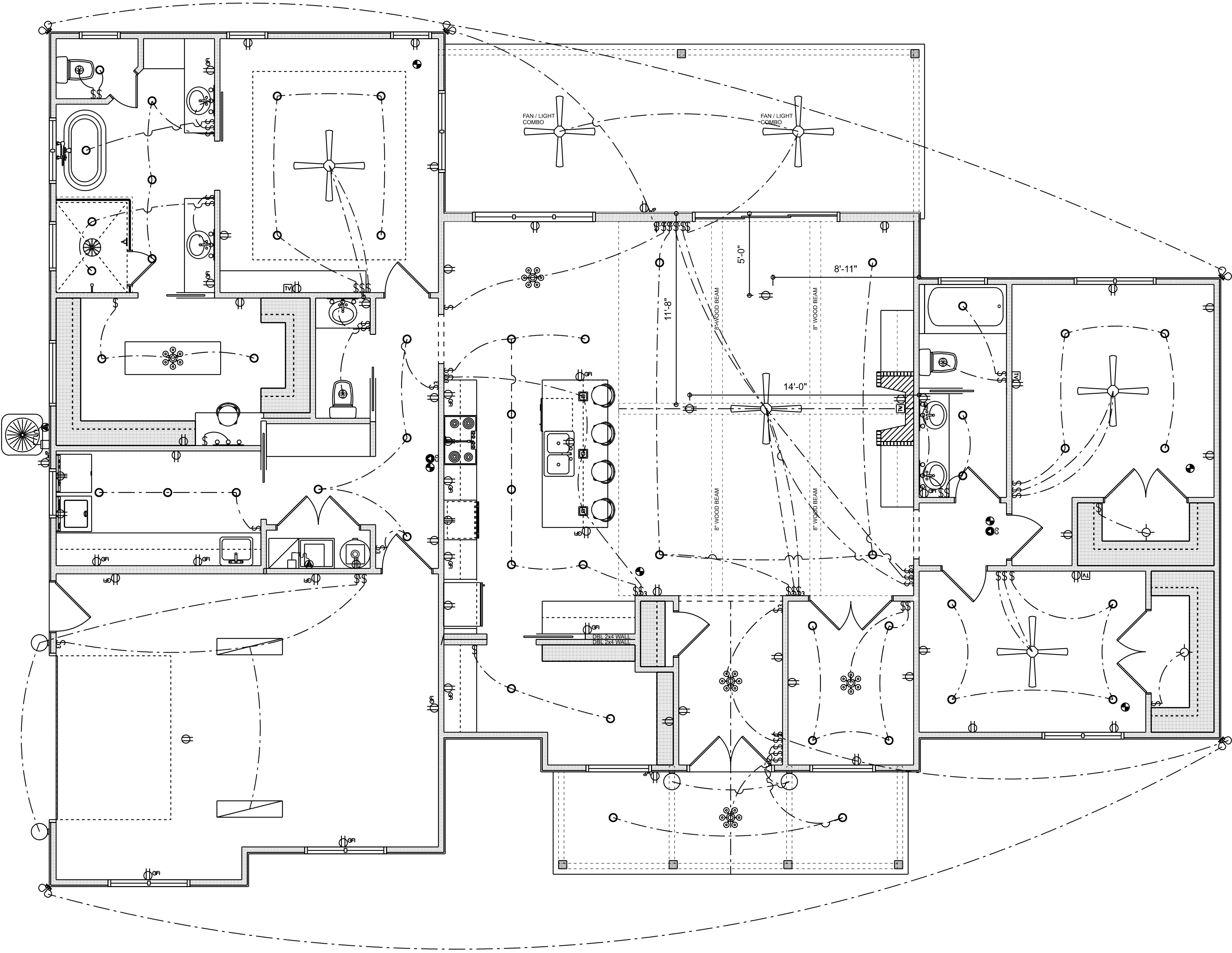
ELECTRICAL PLAN
