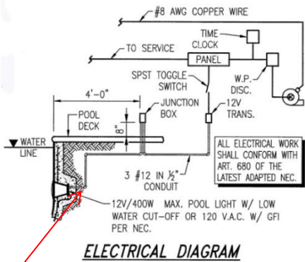
ELECTRICAL DIAGRAM
