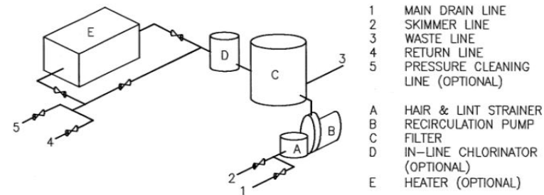
FILTER SYSTEM
