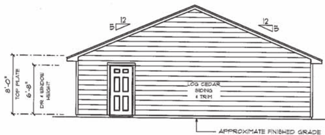
• RIGHT SIDE ELEVATION • SCALE : 1/4" = 1'-0"
