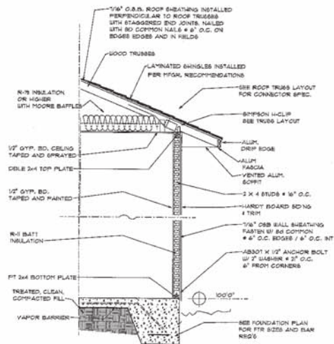
TYPICAL WALL SECTION
