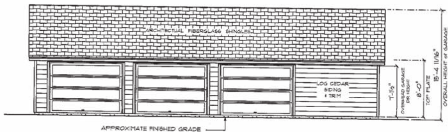
• FRONT ELEVATION • SCALE : 1/4" = 1'-0"
