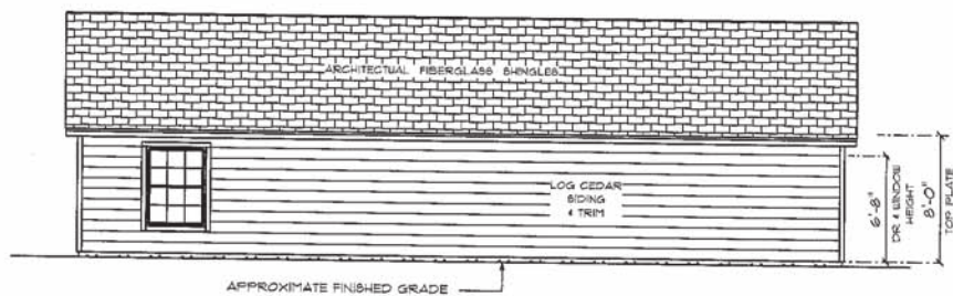
• REAR ELEVATION • SCALE : 1/4" = 1'-0"
