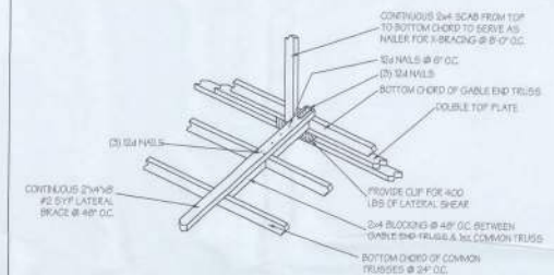
TYPICAL DETAIL ISOMETRIC OF LATERAL BRACE TO GABLE END
