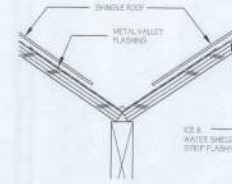
VALLEY FLASHING
