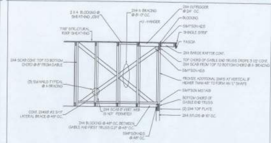
PLATFORM FRAMING TO GABLE END
