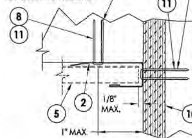
DETAIL "C" J-Channel
