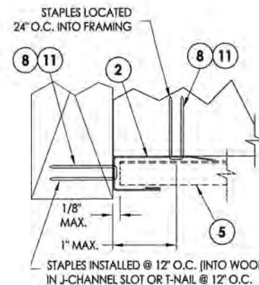
DETAIL "D" J-Channel Fascia
