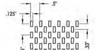
LOUVER PATTERN (LOUVERS FORMED IN SAME DIRECTION AS RIBS)
