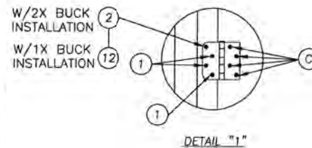
DETAIL "1"
