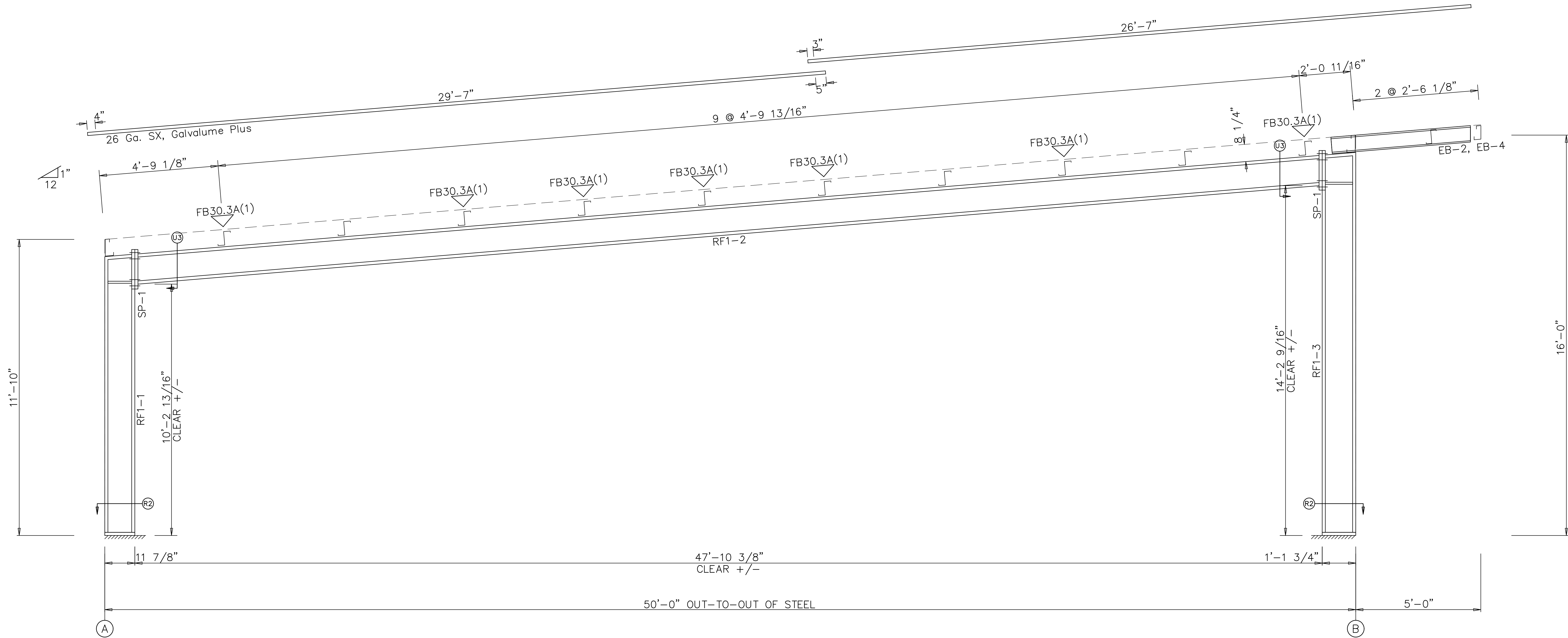
RIGID FRAME ELEVATION: FRAME LINE 1 7
