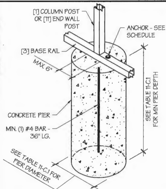
CONCRETE PIER DETAIL SCALE: NTS
