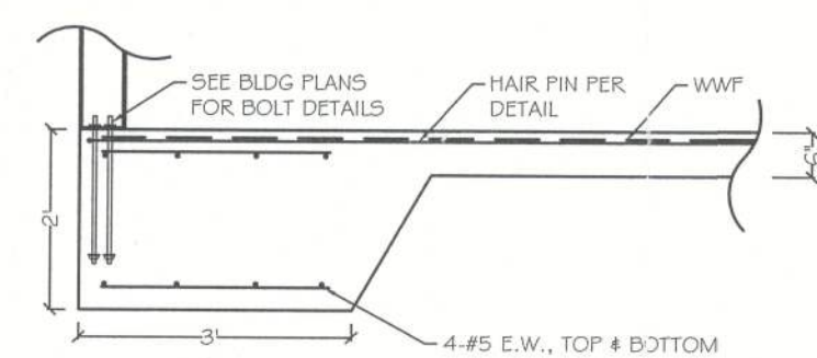
(A) 3'x3'x2' FOOTING DETAIL NOT TO SCALE
