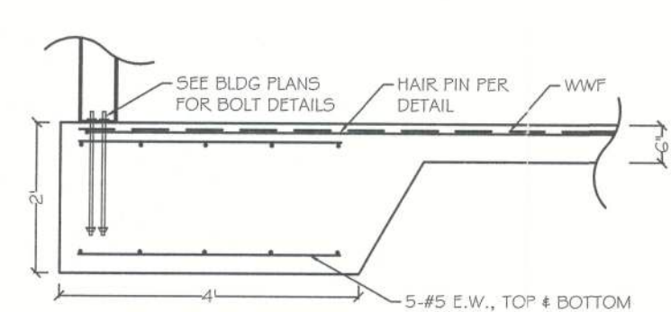
(B) 4'x4'x2' FOOTING DETAIL NOT TO SCALE
