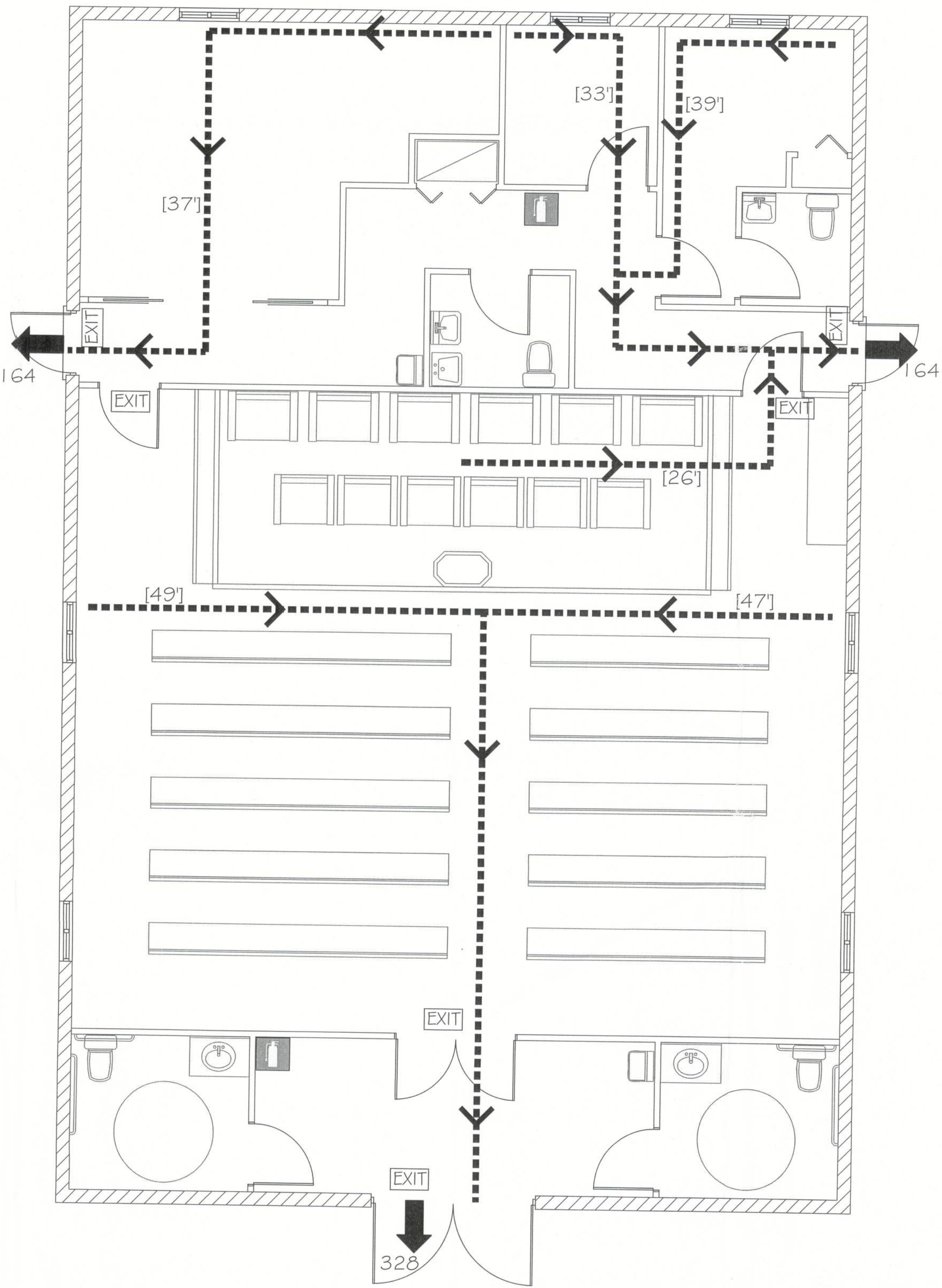
LIFE SAFETY PLAN SCALE: 1/4" = 1'
