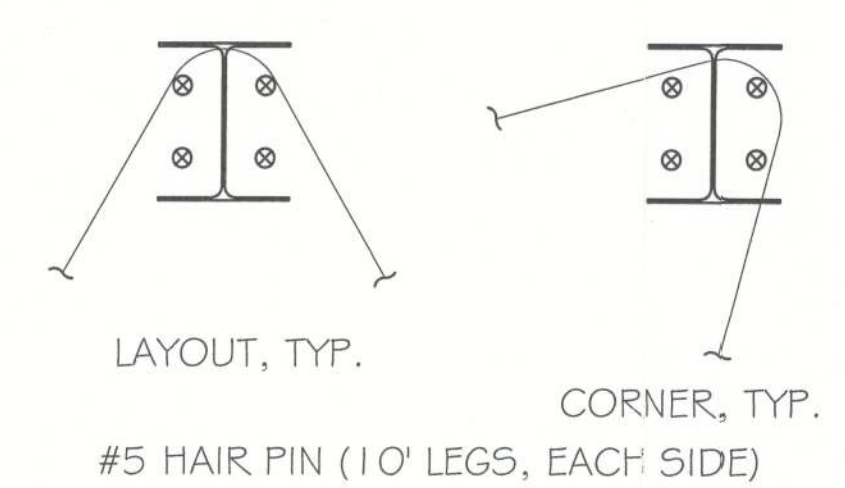
HAIR PIN DETAIL NOT TO SCALE
