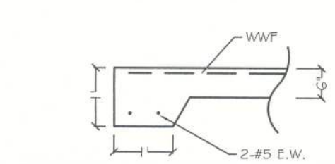
(C) 12" THICKENED EDGE DETAIL NOT TO SCALE
