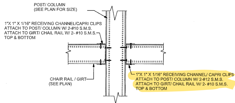
CHAIR RAIL TO POST/ COLUMN CONCEALED CONNECTION NTS
