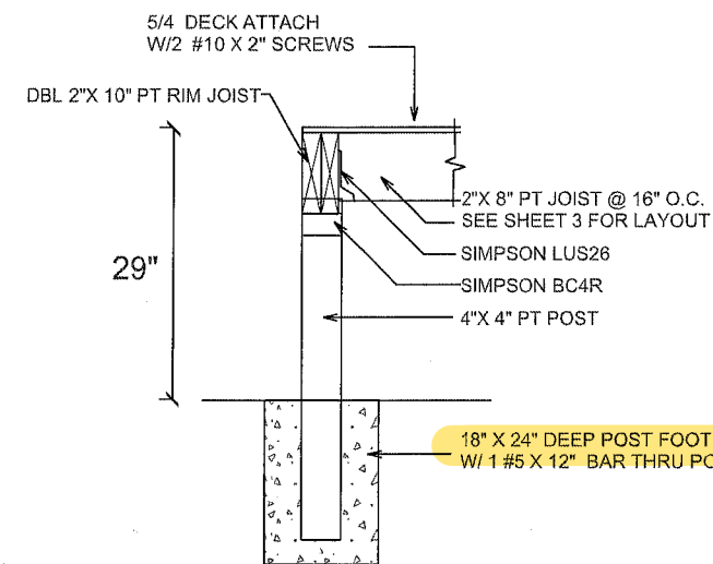
POST FOOTING TO DECK
