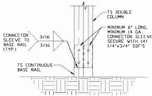
POST/BASE RAIL CONNECTION DETAIL SCALE: NTS
